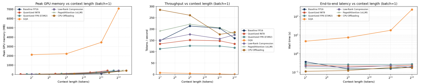
Fig. 2. Measured behaviour of the seven directly-run techniques as the context length grows at batch=1 (3 trials averaged). Left: peak GPU memory versus context length. The tiny-gpt2 techniques (FP16 baseline, INT8, FP8, low-rank, PagedAttention, CPU Offloading) stay between 9.8 MB and 402 MB; their curves overlap because the tiny-gpt2 KV cache is at most 0.06 MB while weights and activations dominate, so cache-size differences are invisible at this scale. GQA (TinyLlama-1.1B) is the heaviest (2.1–7.1 GB) and grows fastest with context. The analytical simulators are omitted from this panel because they allocate no memory (their cache sizes are shown in Figure 4). Centre: throughput in tokens per second; CPU Offloading (177–285) and PagedAttention (178–221, via its pure-PyTorch CPU fallback, marked with \times ) lead, followed by the FP16 baseline (149–213), low-rank (151–177), INT8 (135–152), and FP8 (113–126), and GQA is slowest (0.1–6.9) because TinyLlama-1.1B is two orders of magnitude larger than tiny-gpt2. Right: end-to-end latency on a log scale; GQA's 5–238 s dominates the axis, while the tiny-gpt2 techniques stay below 0.4 s.
