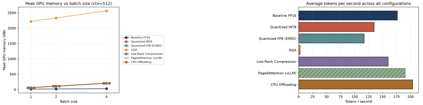
Fig. 3. Measured behaviour of the seven directly-run techniques across batch sizes and an aggregated throughput summary (3 trials averaged). Left: peak GPU memory at context_length=512 as the batch grows from 1 to 4; the tiny-gpt2 techniques scale from 15–60 MB (batch 1) to 29–206 MB (batch 4), and GQA (TinyLlama-1.1B) from 2.2 GB to 2.6 GB. Right: average tokens per second across all (context, batch) configurations; CPU Offloading (204) and PagedAttention (190, CPU fallback) lead, followed by the FP16 baseline (176), low-rank compression (160), INT8 (135), and FP8 (117); GQA is at the low end (2.8) because it runs the much larger TinyLlama-1.1B.
