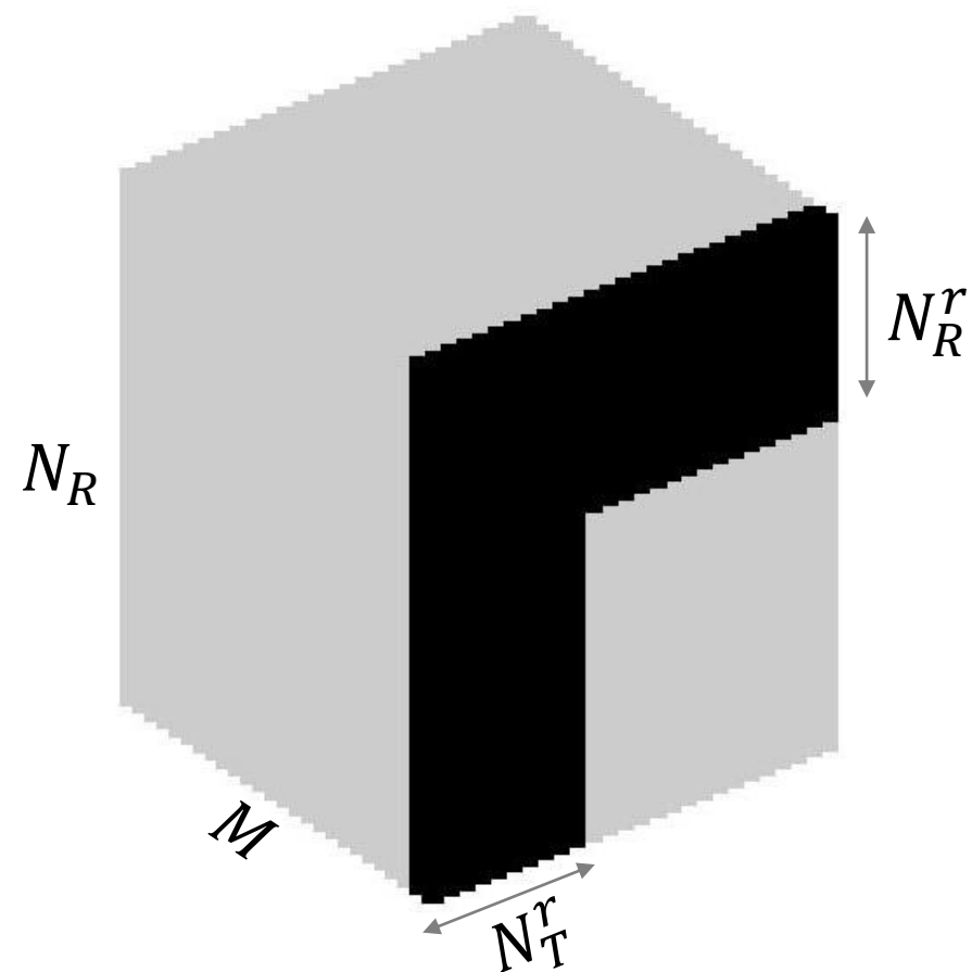
(c) The Reduced Rank MRC Detection lower the complexity count of the HL-ML and the MRC detectors approximately by (N_T - N_T^r)(N_R - N_R^r)
