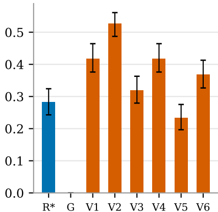
Demographic parity diff.
