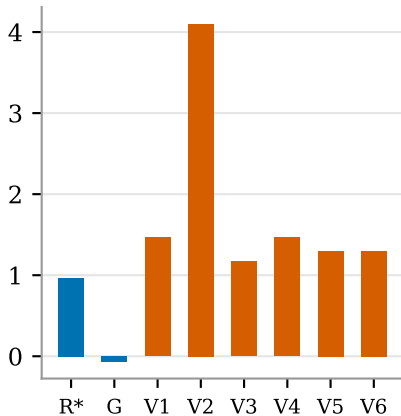
Accuracy drop, char-swap (pp)
