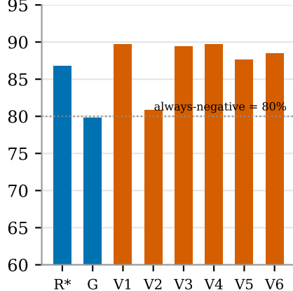
Clean accuracy (%)
