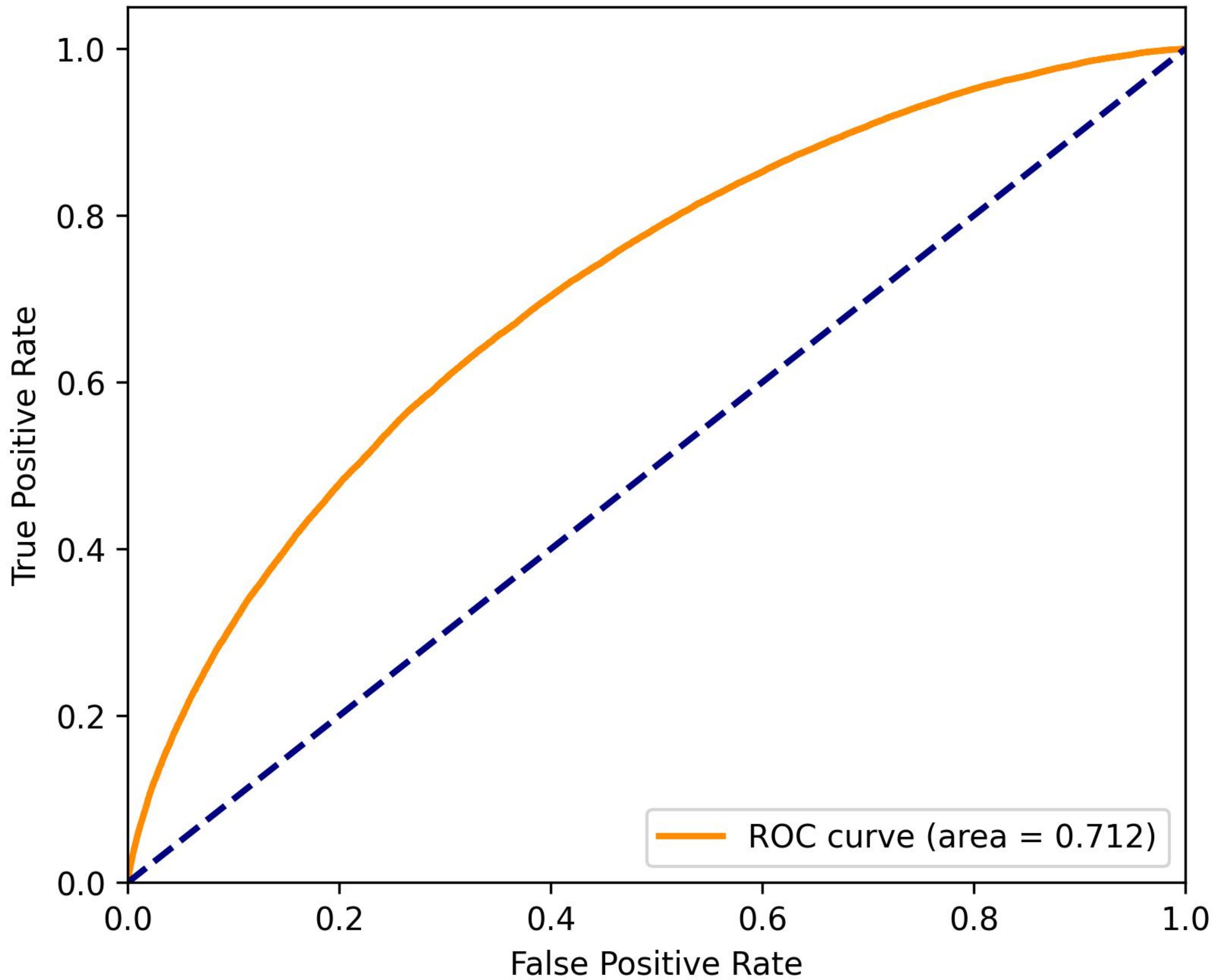
ROC Curve: LogisticRegression
