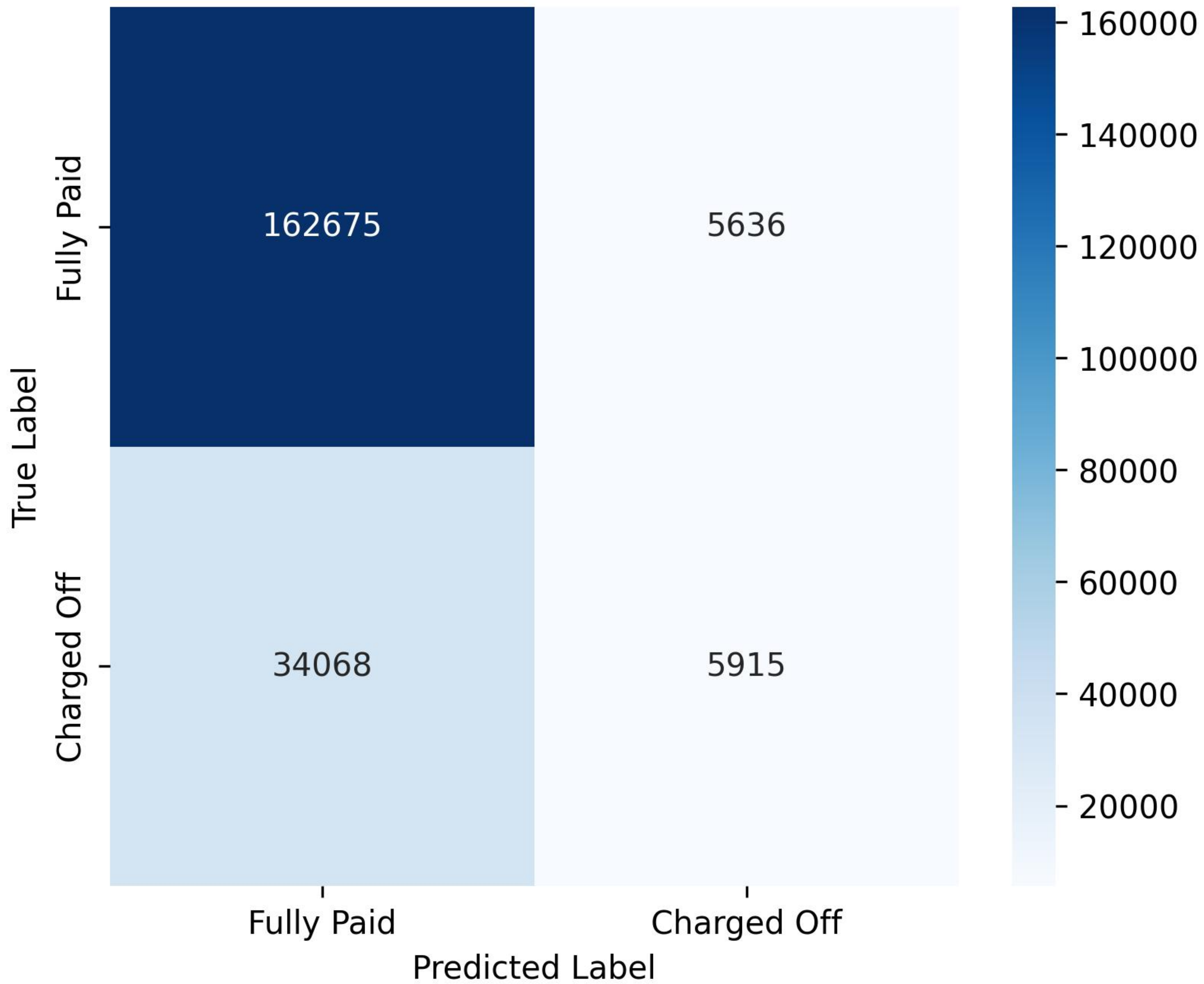
Confusion Matrix: SVM
