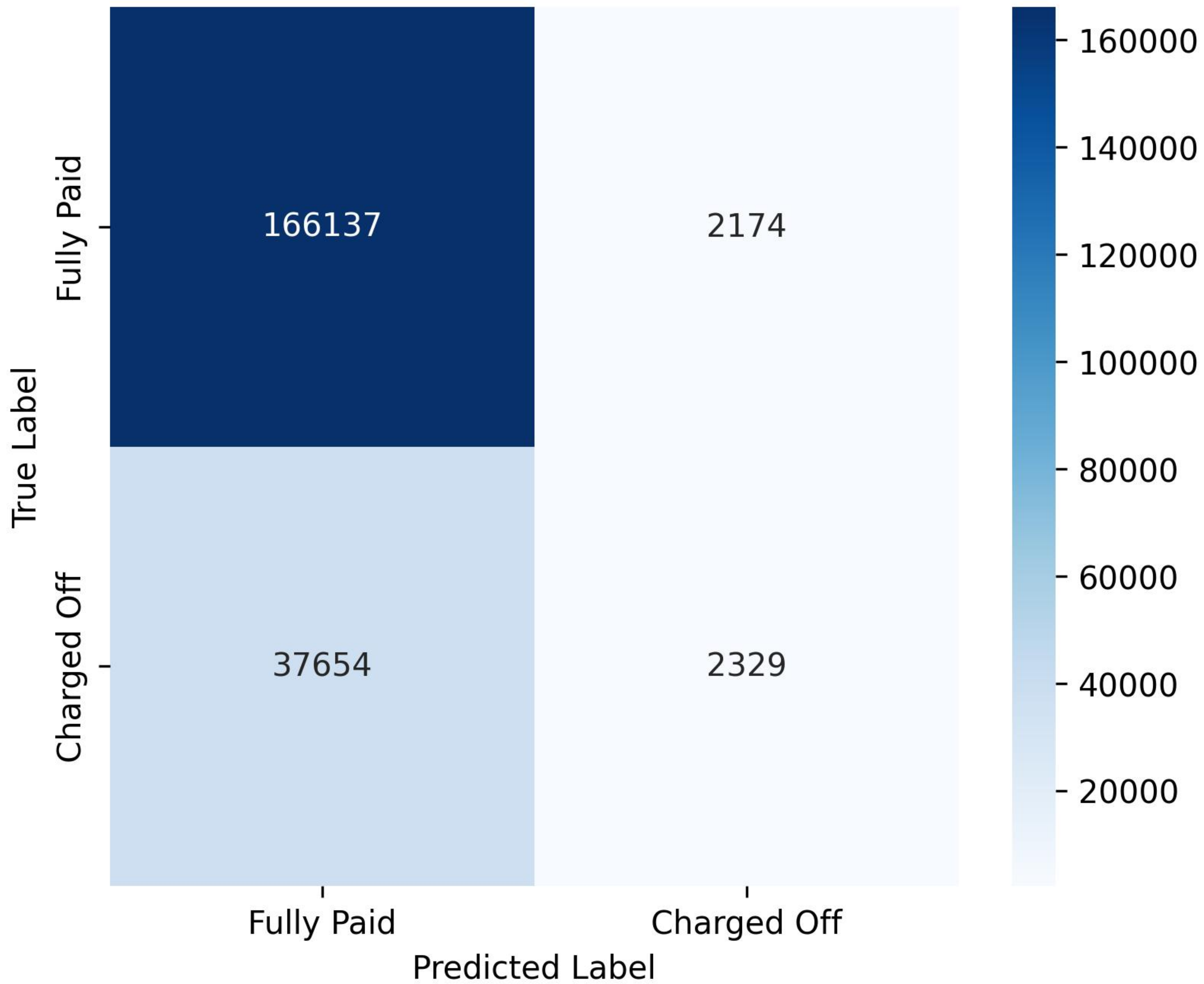
Confusion Matrix: KNN
