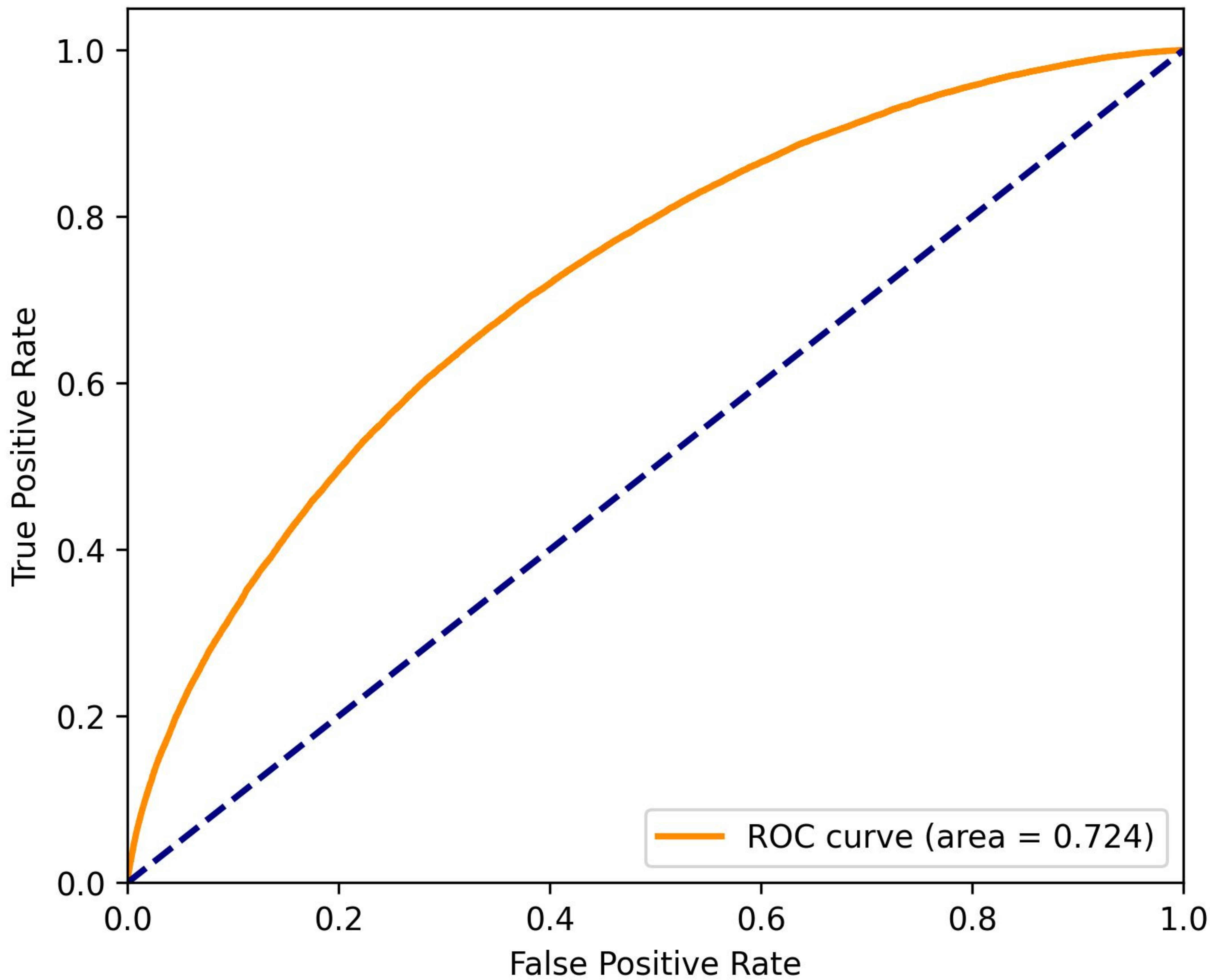
ROC Curve: XGBoost
