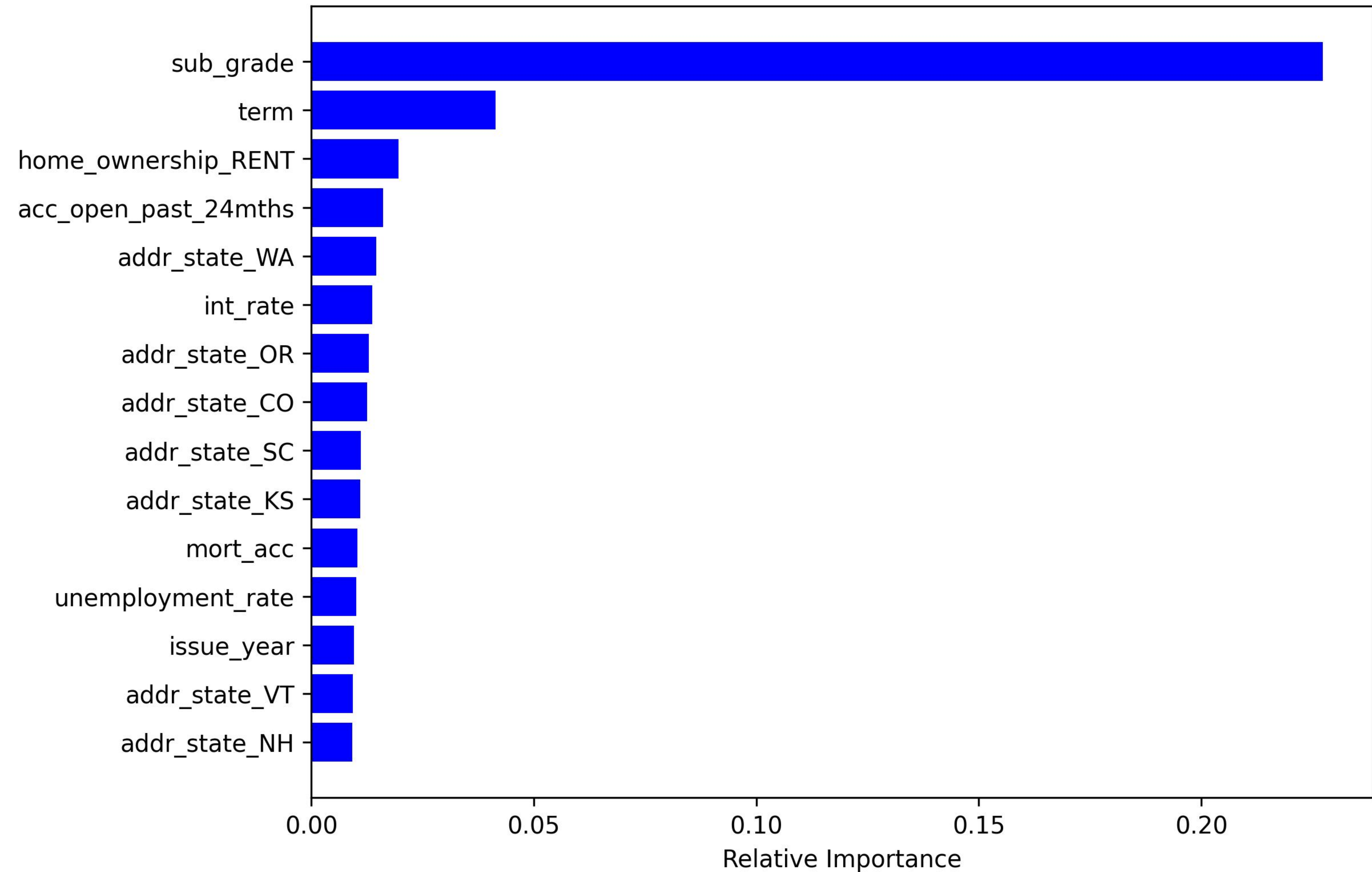
Top 15 Feature Importances: XGBoost
