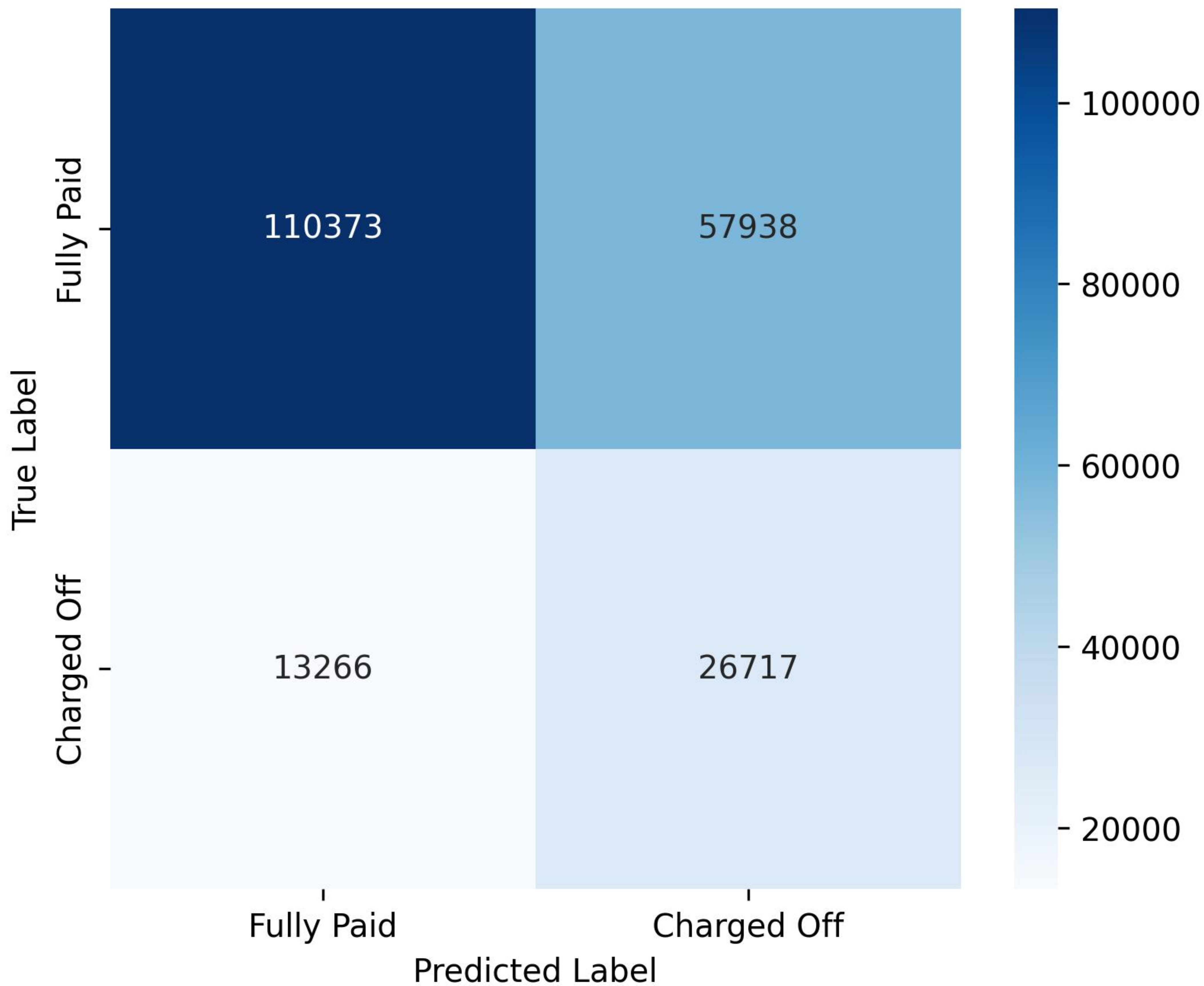
Confusion Matrix: XGBoost
