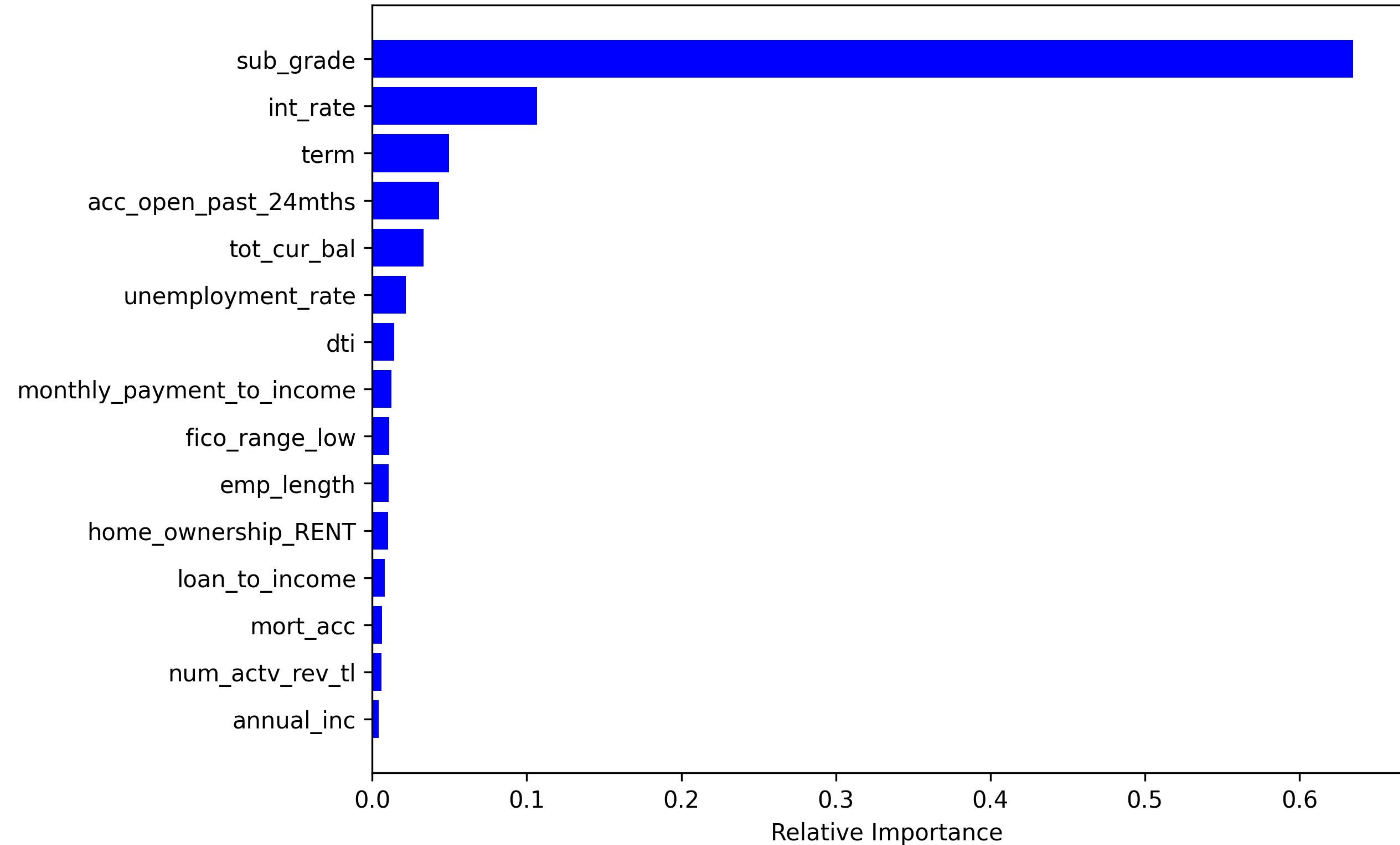
Top 15 Feature Importances: DecisionTree
