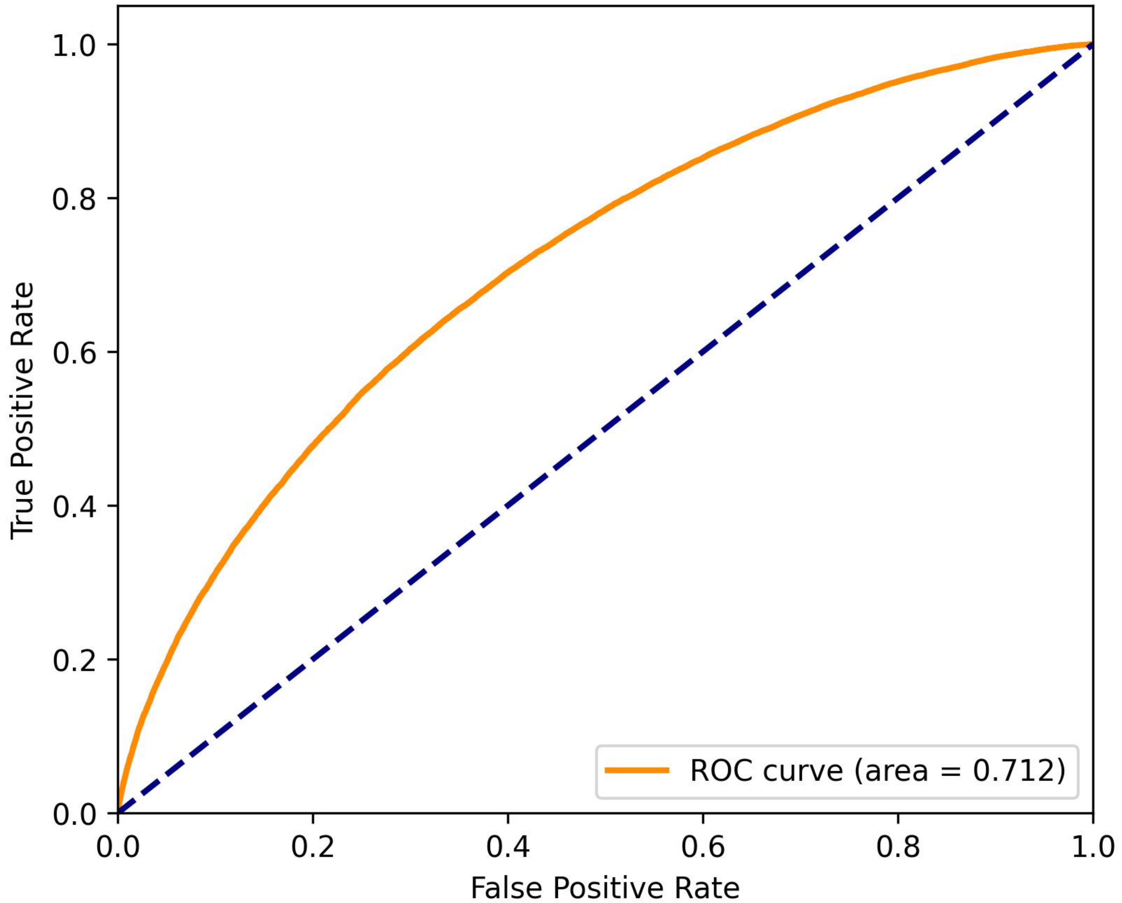
ROC Curve: SVM
