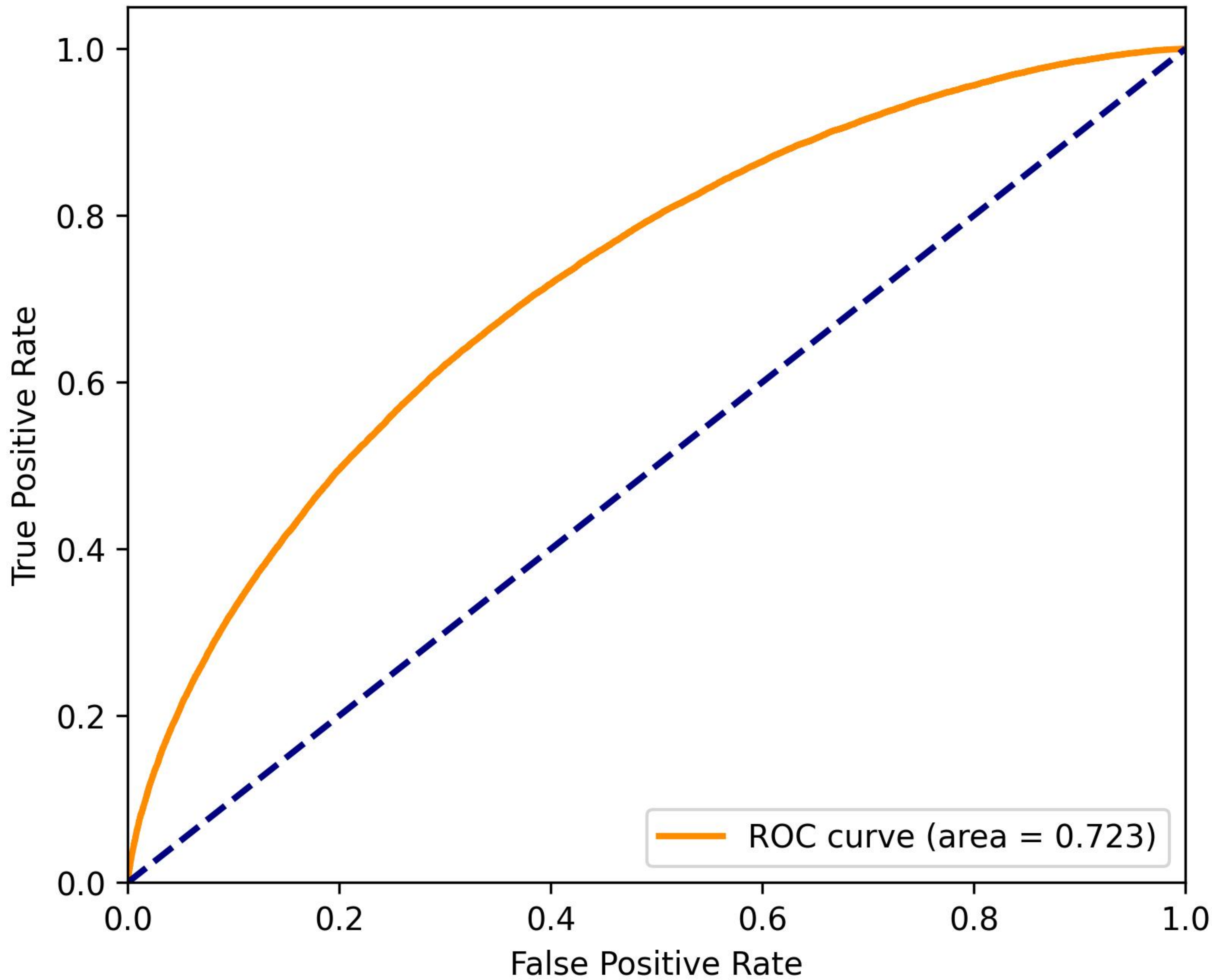
ROC Curve: HistGradientBoosting
