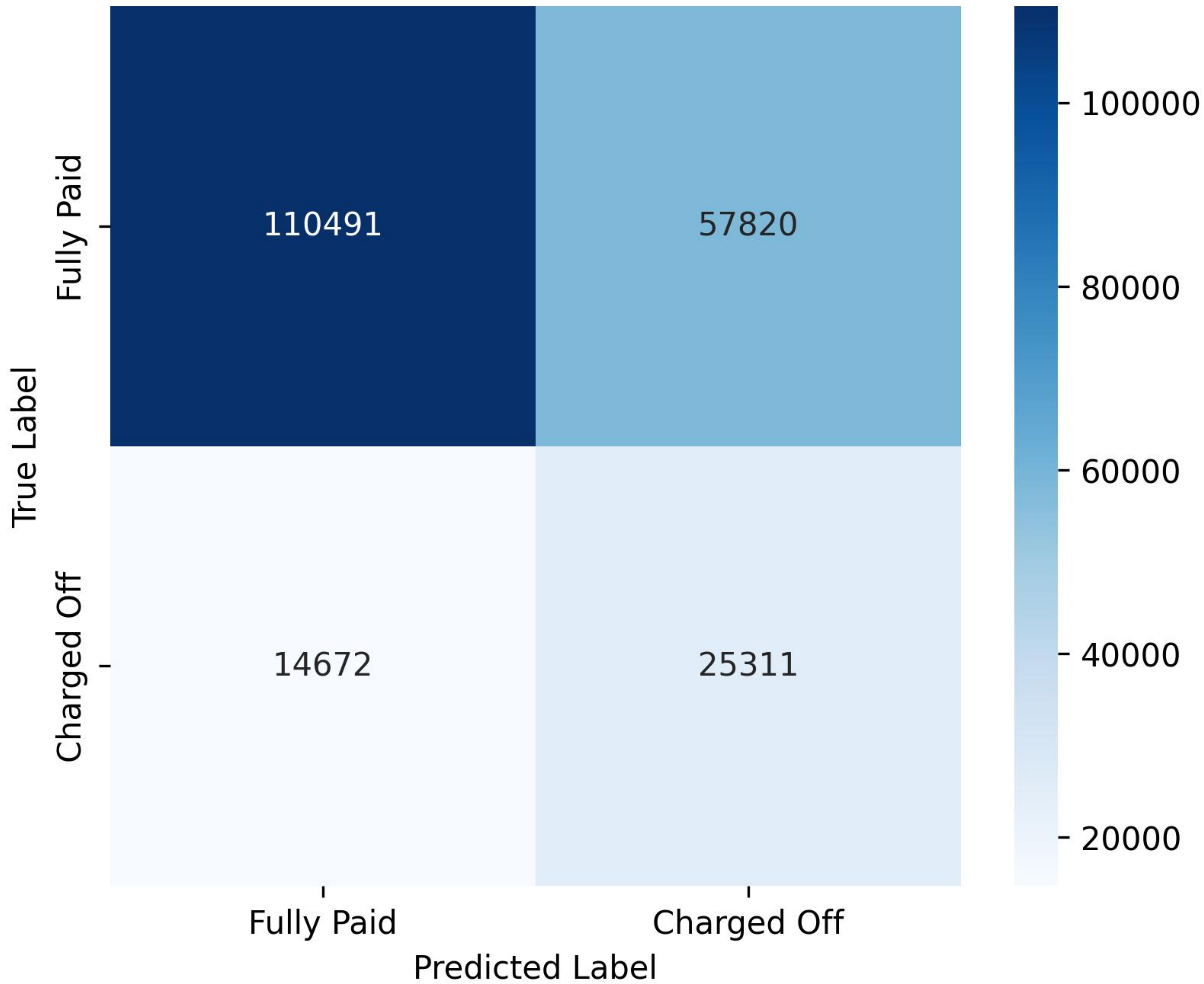
Confusion Matrix: DecisionTree
