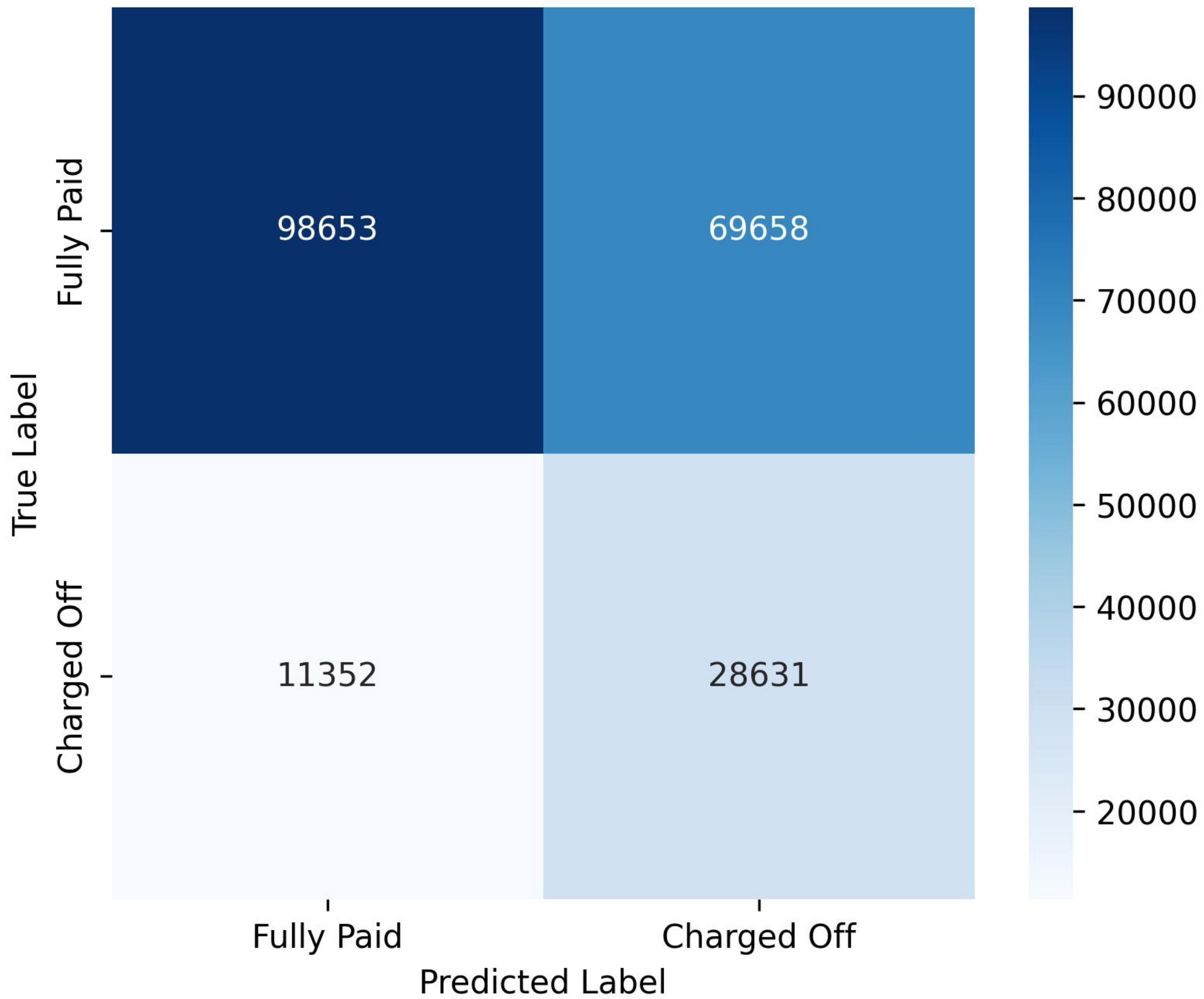
Confusion Matrix: LogisticRegression
