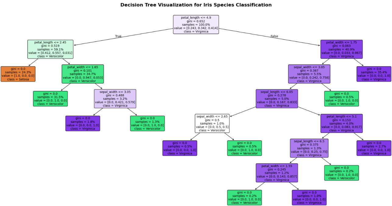
Fig: Decision Tree Visualization
