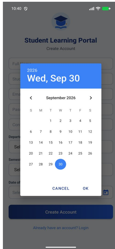
Fig 2: Calendar DatePickerDialog
