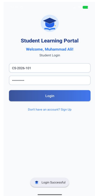
Fig 13: 'Login Successful'
