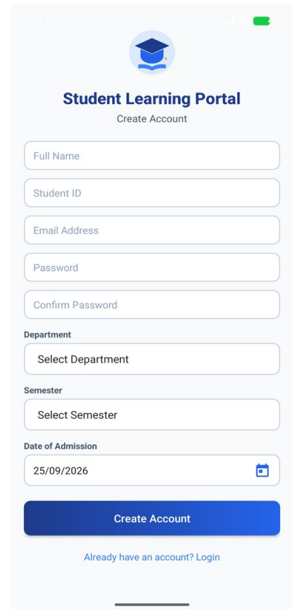
Fig 3: Date Populated (25/09/2026)
