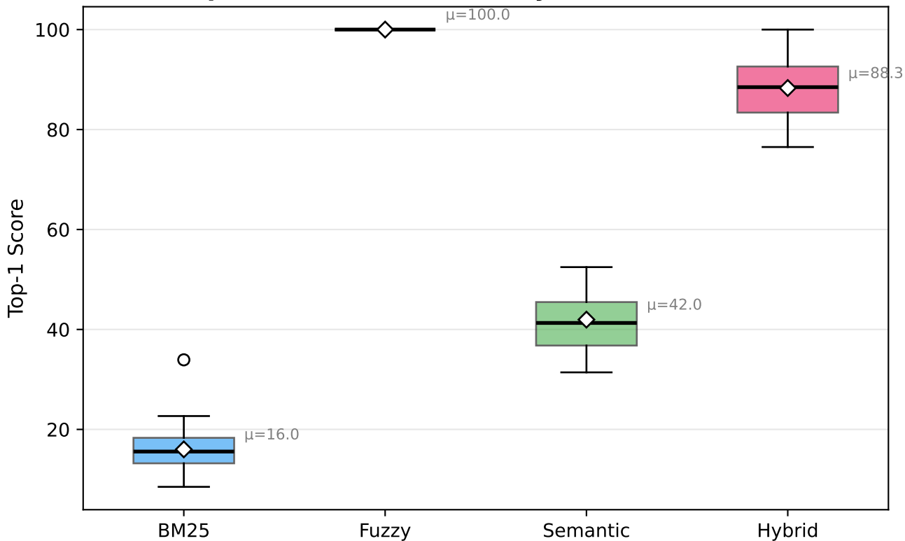
Top-1 Score Distribution by Retrieval Method
