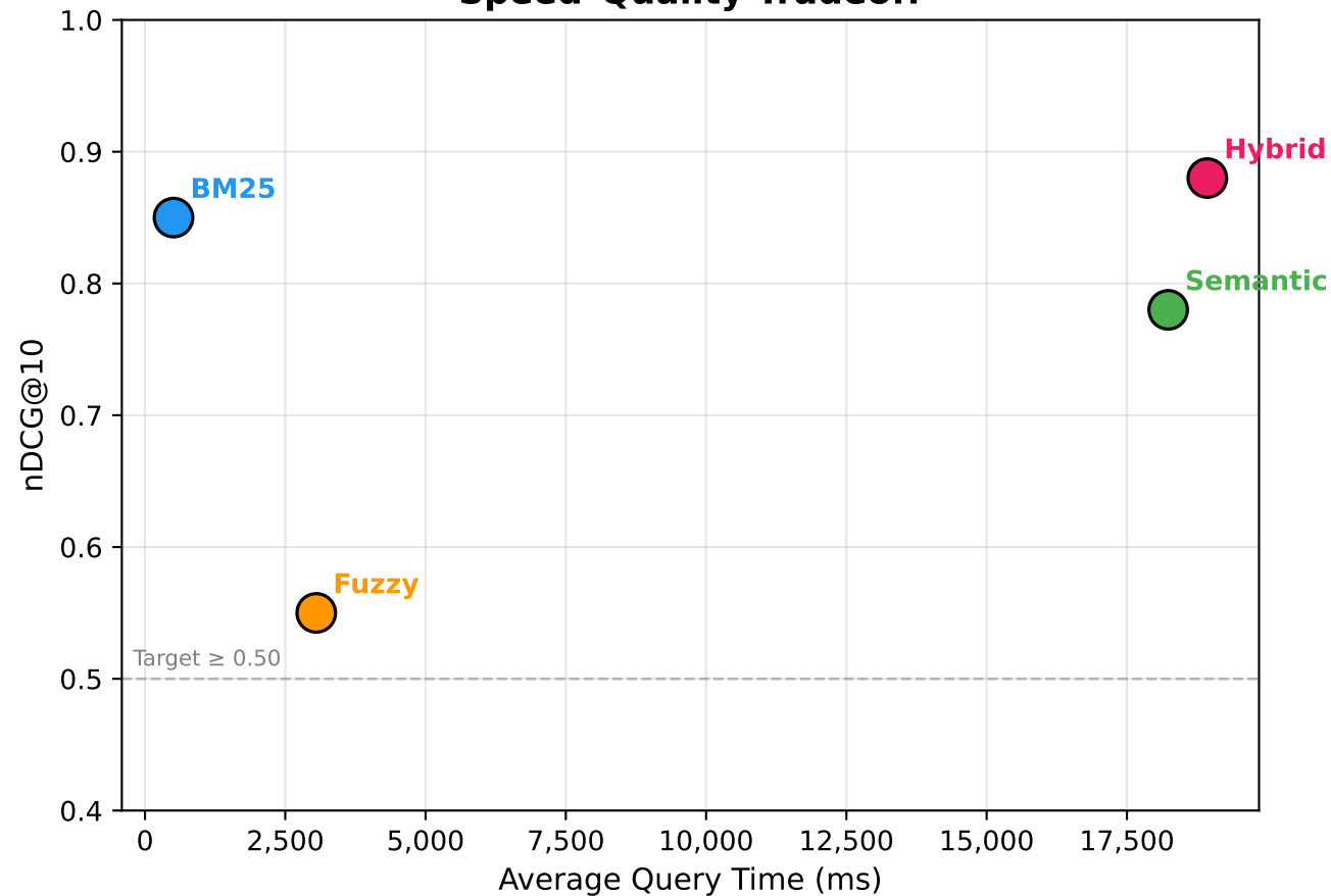
Speed-Quality Tradeoff
