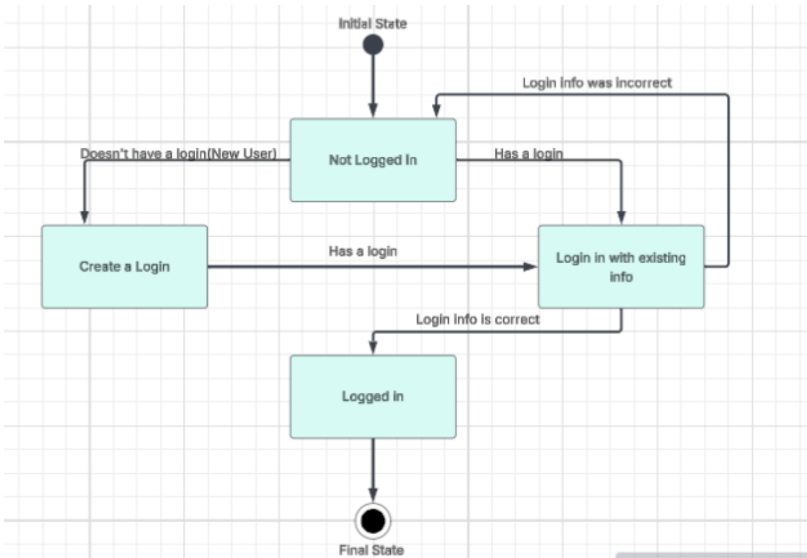
Figure 3: State Diagram
