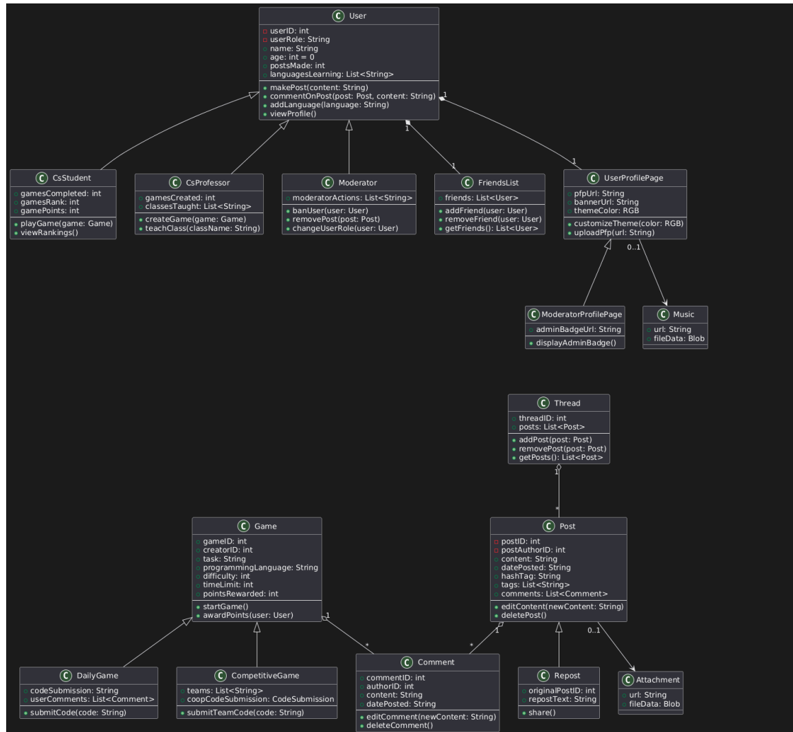
Figure 1: Class Diagram
