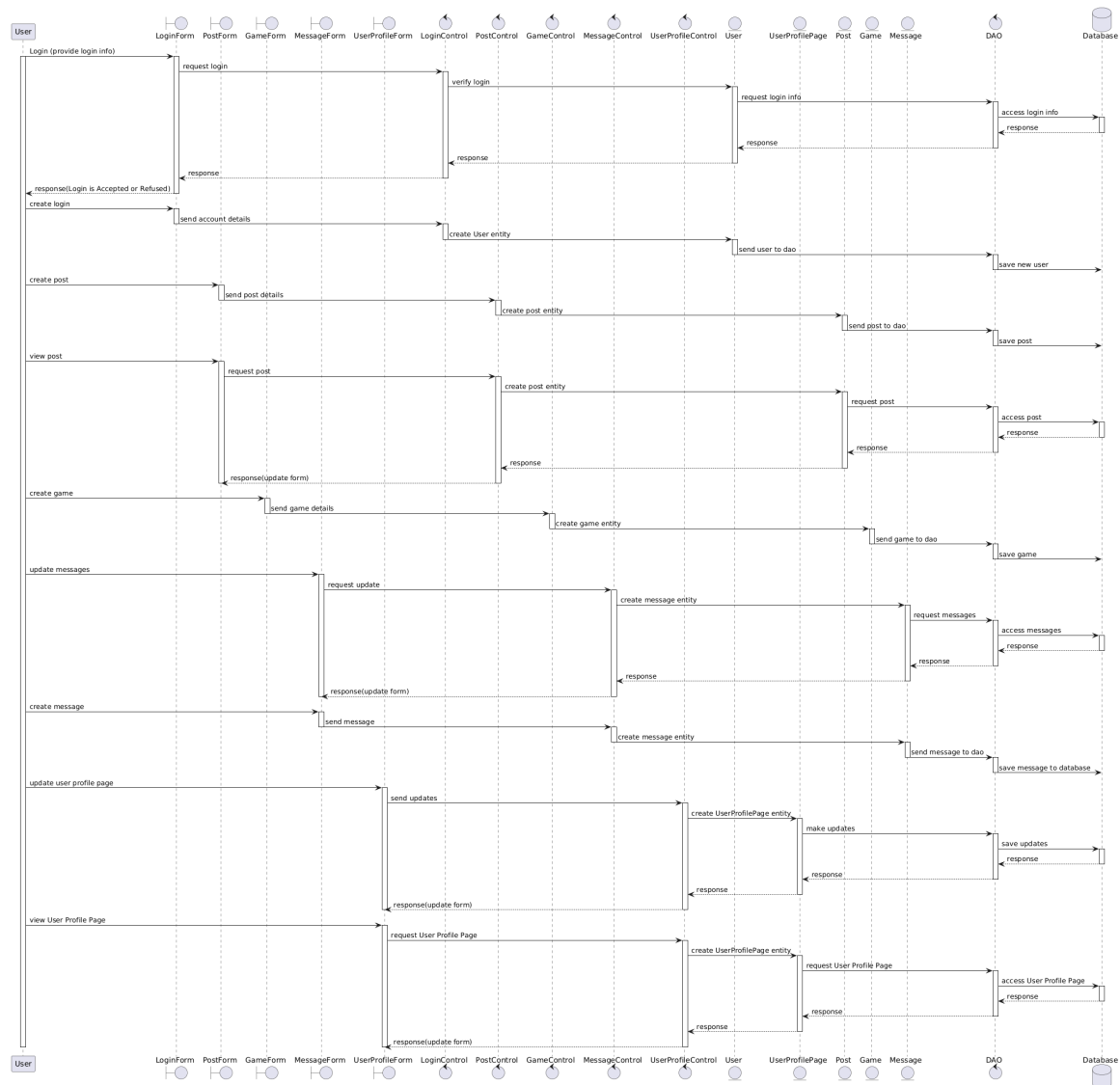
Figure 2: Sequence Diagram
