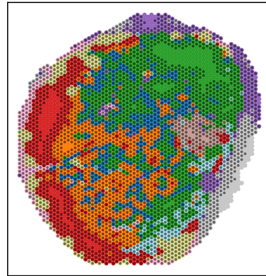
UNIFORM_ALL seed 2
