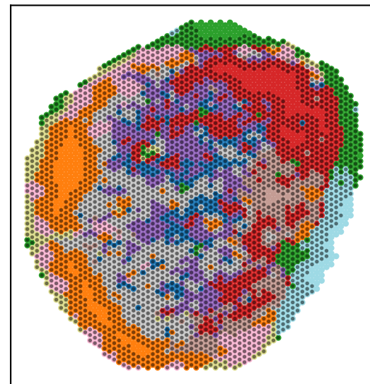
UNIFORM_ALL seed 0
