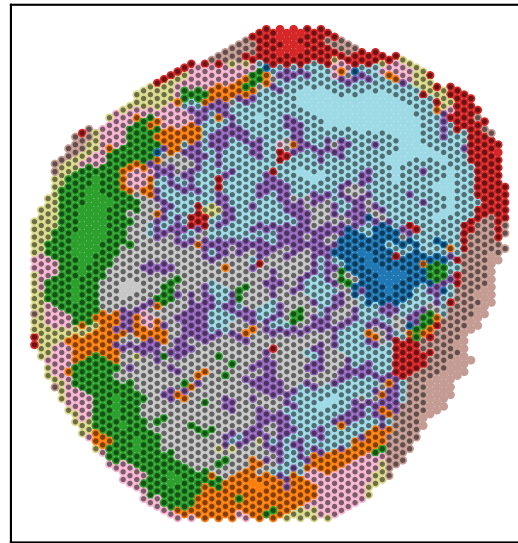
UNIFORM_CROSS seed 2
