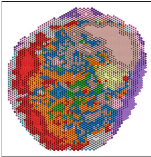
UNIFORM_WITHIN seed 2
