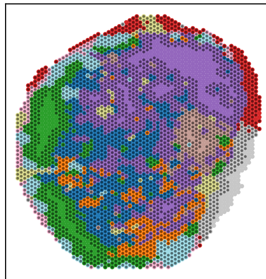
UNIFORM_CROSS seed 0
