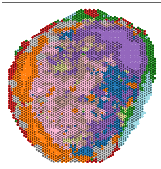
UNIFORM_WITHIN seed 0
