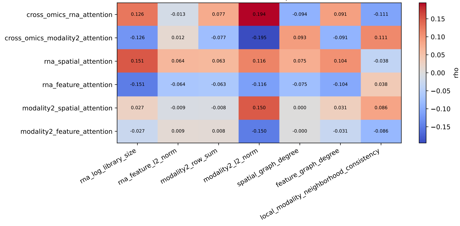
Attention / label-free QC Spearman rho
