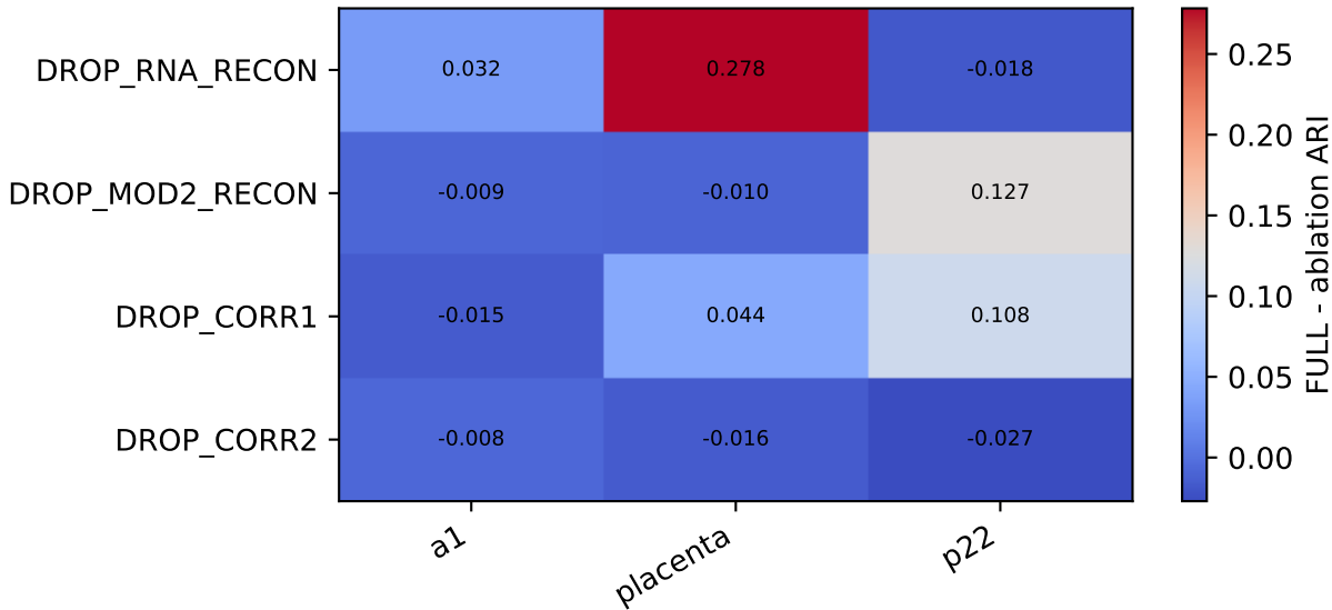
Loss-term ablation mean ARI delta
