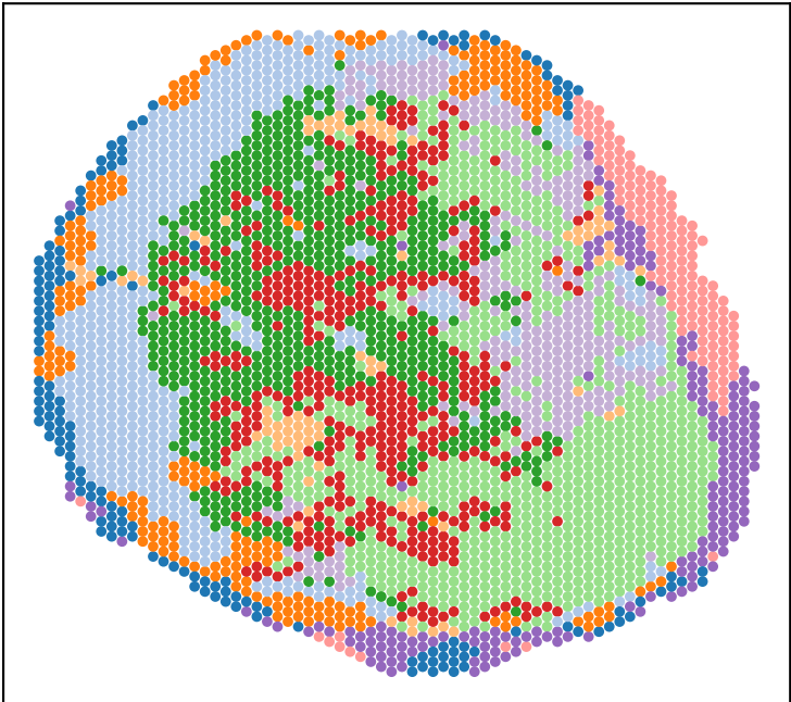
UNIFORM_WITHIN seed 0
