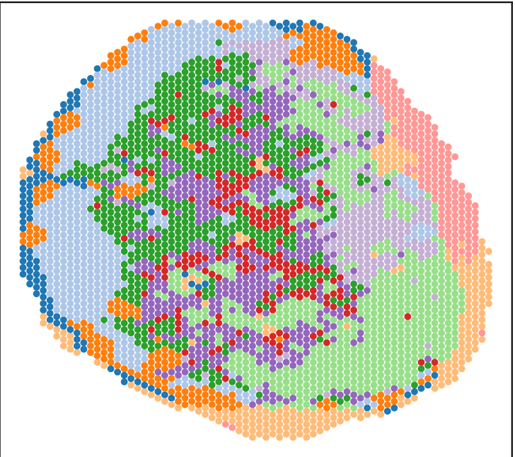
UNIFORM_ALL seed 0
