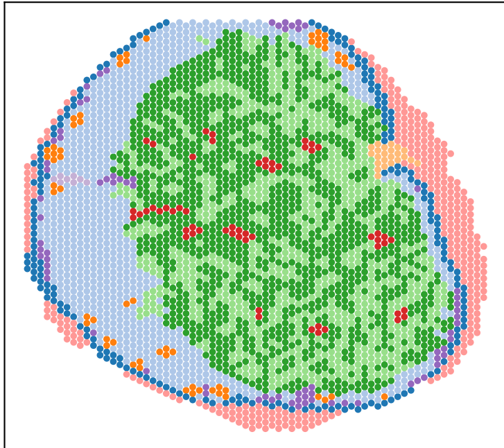
Ground truth
