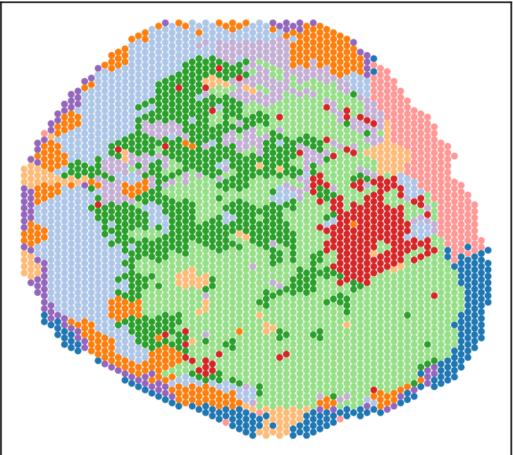
UNIFORM_CROSS seed 0
