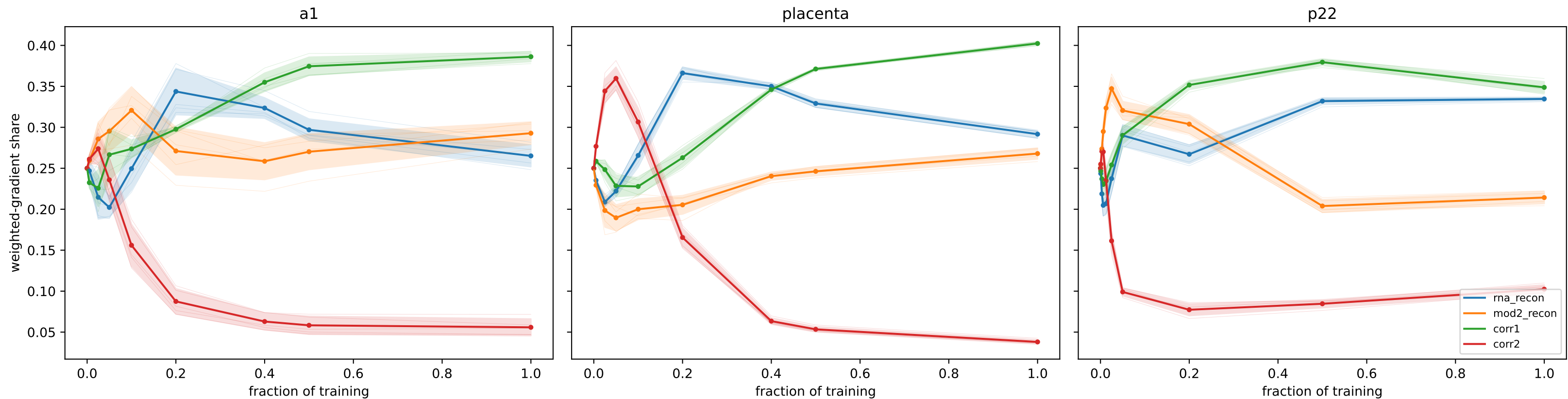
IGE weighted-gradient trajectories: mean \pm seed SD with individual seed traces
