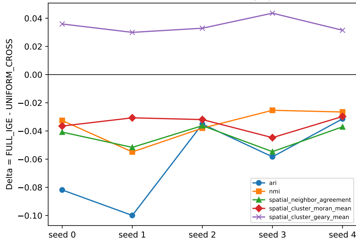
Uniform cross is favored across accuracy/spatial directions
