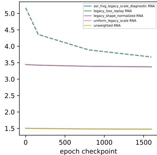
RNA (solid) / modality-2 (dashed); n=5 fixed model seeds; means only placenta
