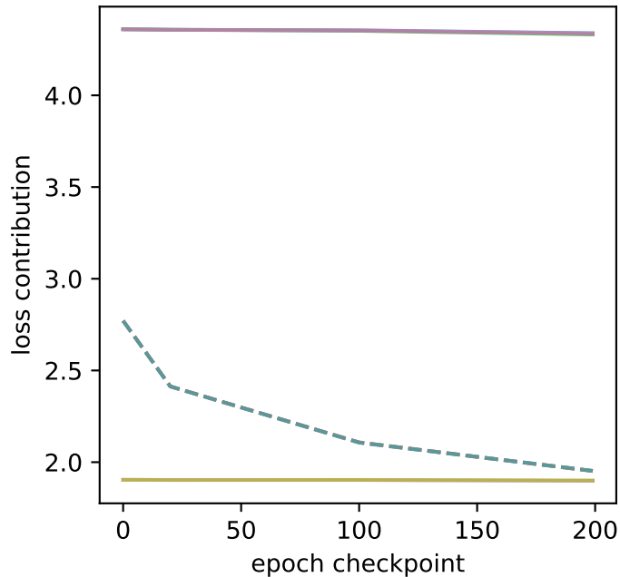
RNA (solid) / modality-2 (dashed); n=5 fixed model seeds; means only placenta
