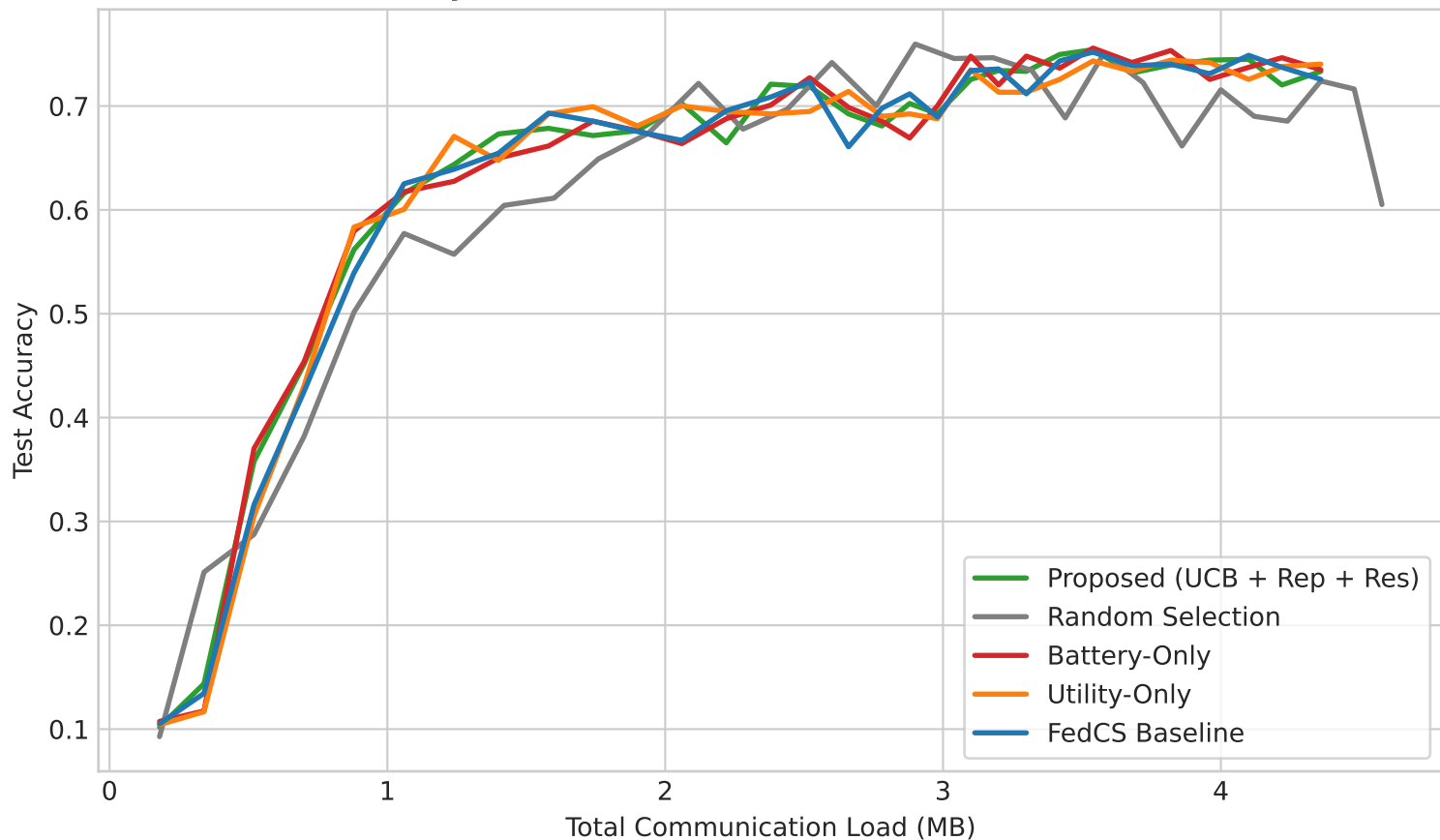
Accuracy vs. Communication Cost (IoT Clients N=14)
