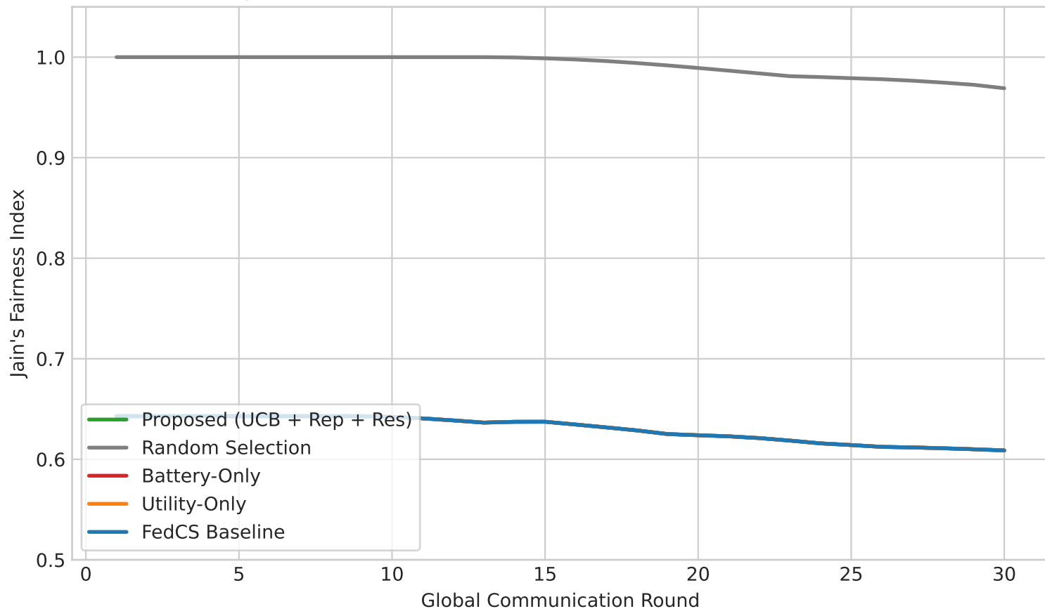
Jain's Fairness Index Evolution (IoT Clients N=14)
