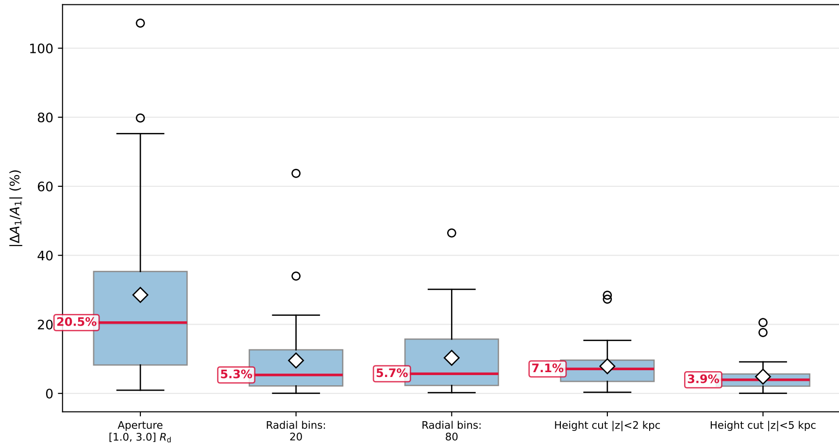
Systematic uncertainty budget (N = 30 TNG50 galaxies)
