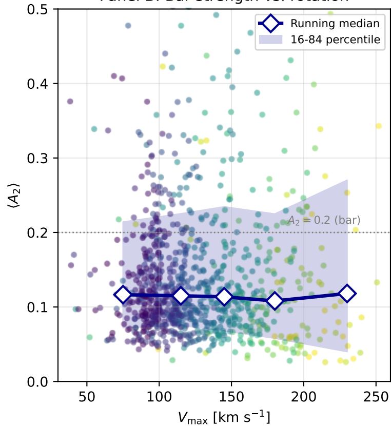
Panel B: Bar strength vs. rotation
