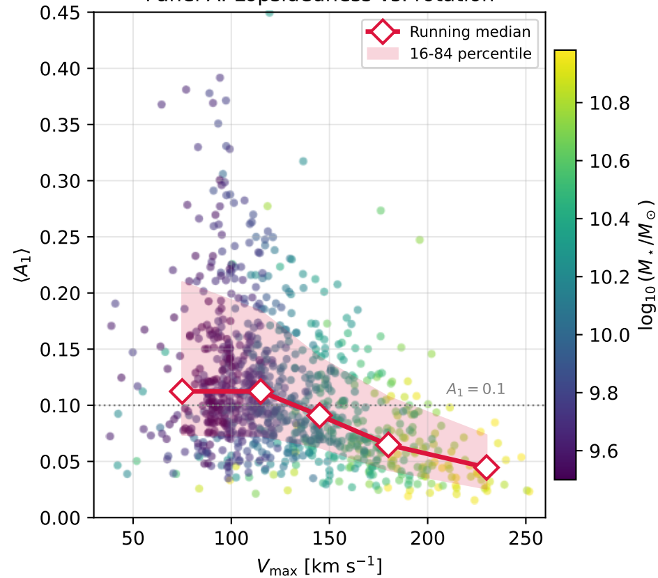
Panel A: Lopsidedness vs. rotation
