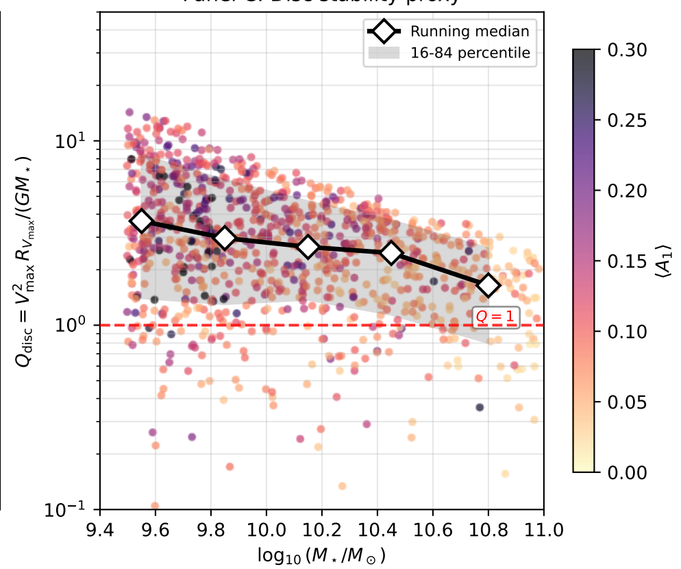
Panel C: Disc stability proxy
