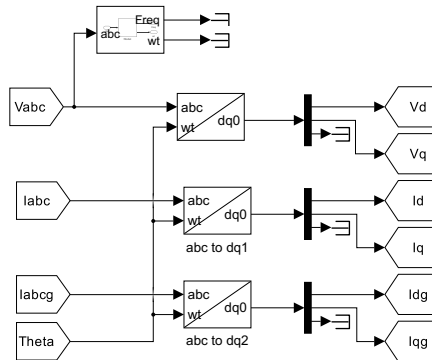
Figure 4: Signal Transformation Subsystem ( abc to dq0 ).
