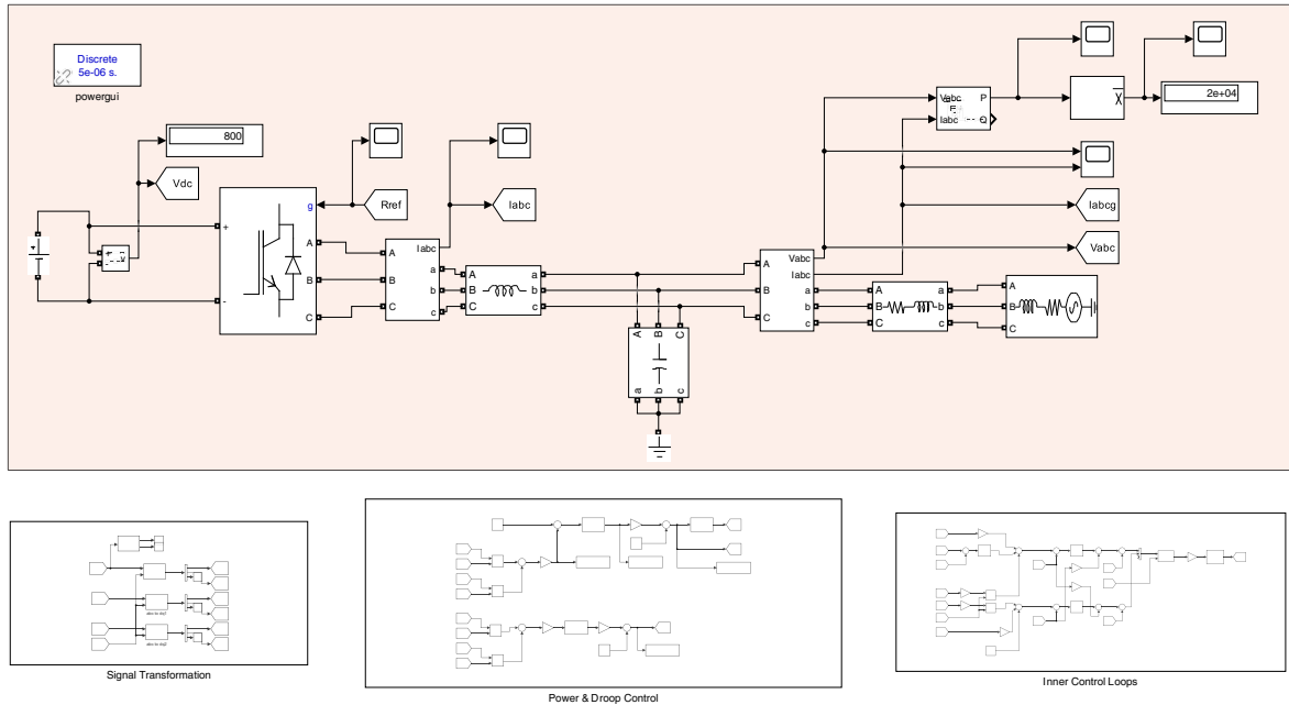
Figure 1: Overall Architecture of the Grid-Forming Inverter System.
