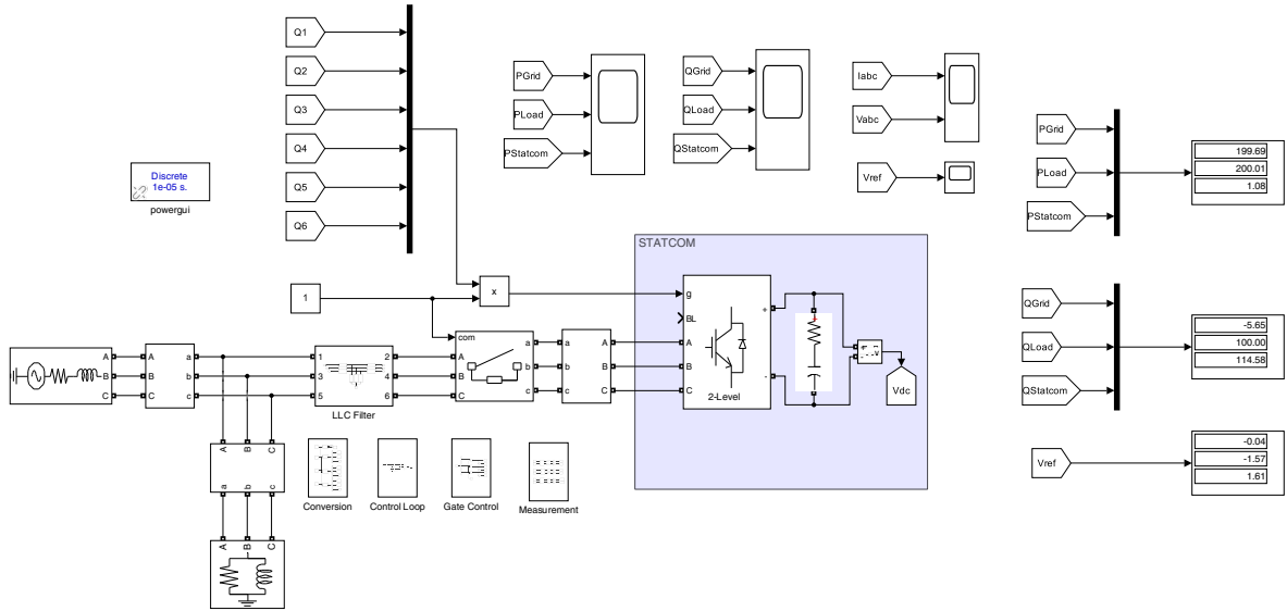
Figure 1: Overall Architecture of the Grid-Connected STATCOM System.
