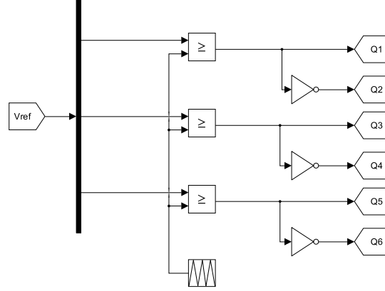
Figure 4: Gate Control Subsystem utilizing SPWM at 10 kHz.
