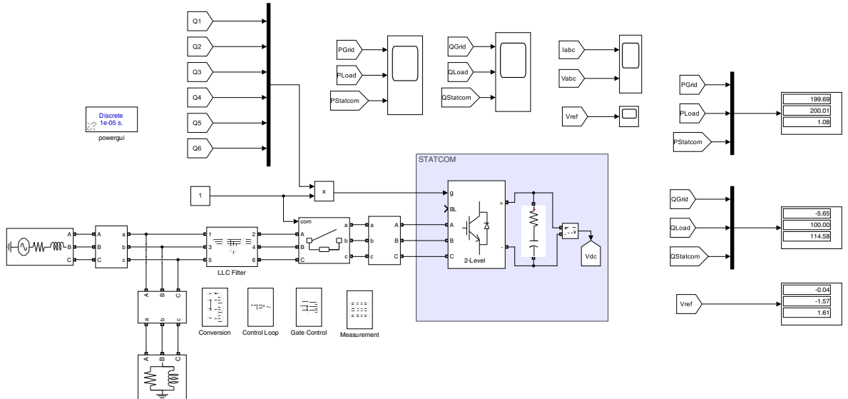
Figure 1: Overall Architecture of the Grid-Connected STATCOM System.
