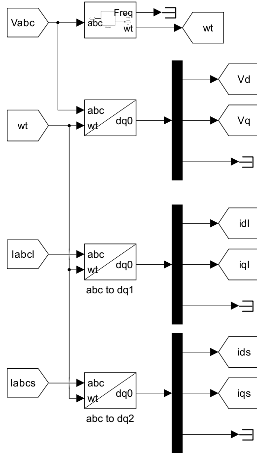
Figure 2: Coordinate Transformation Subsystem ( abc to dq0 ).
