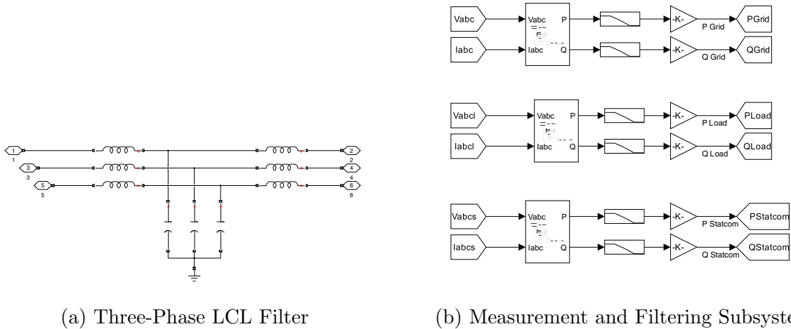
Figure 5: Grid Interfacing Filter and Measurement Architecture.
