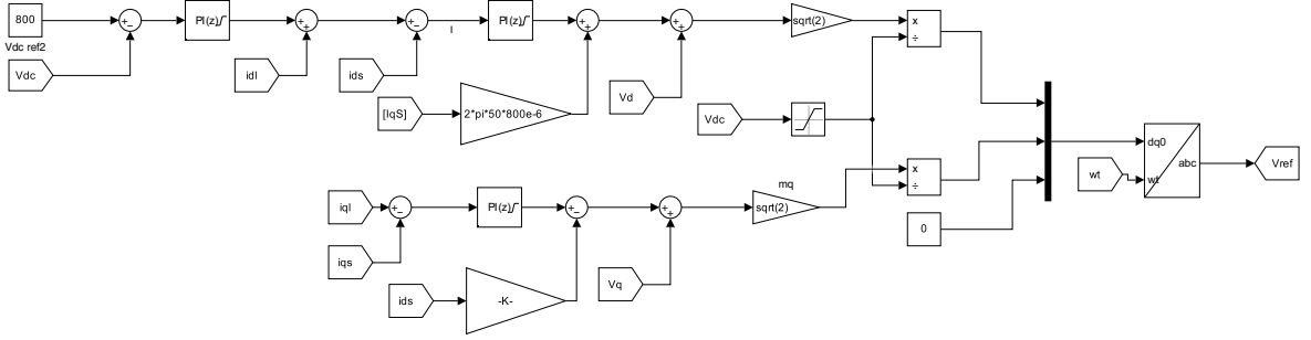
Figure 3: The dq0 Control Loop Subsystem showing PI controllers and Transformations.
