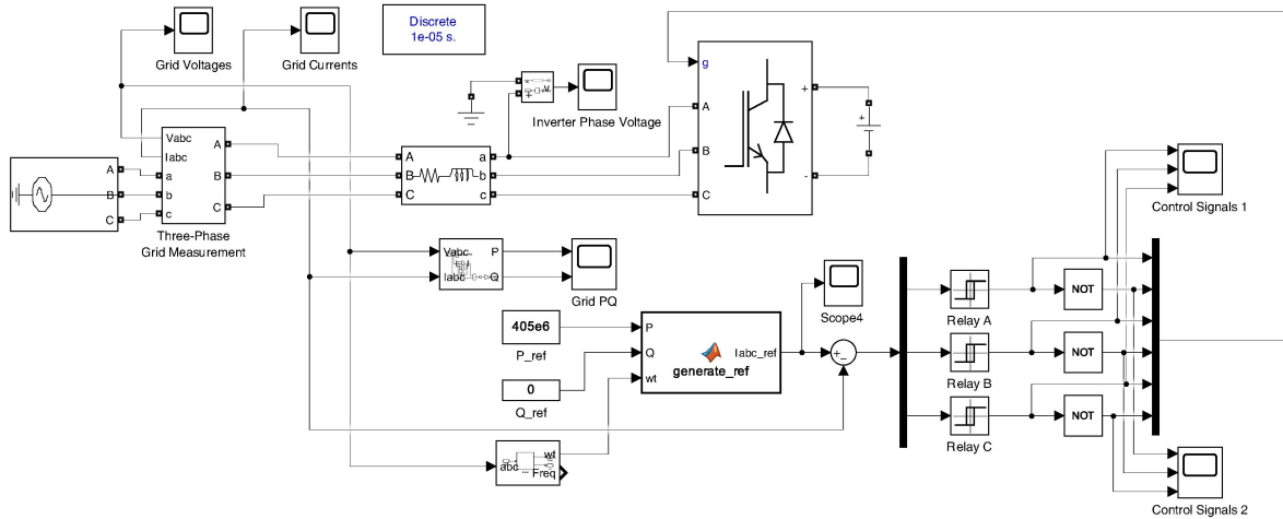
Figure 1: Complete Simulink Model of the Two-Level VSC System.
