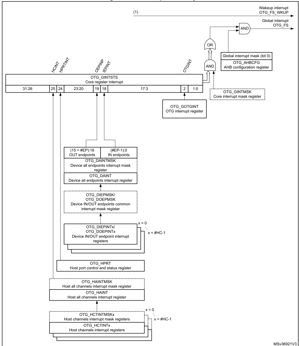
Figure 311. Interrupt hierarchy
