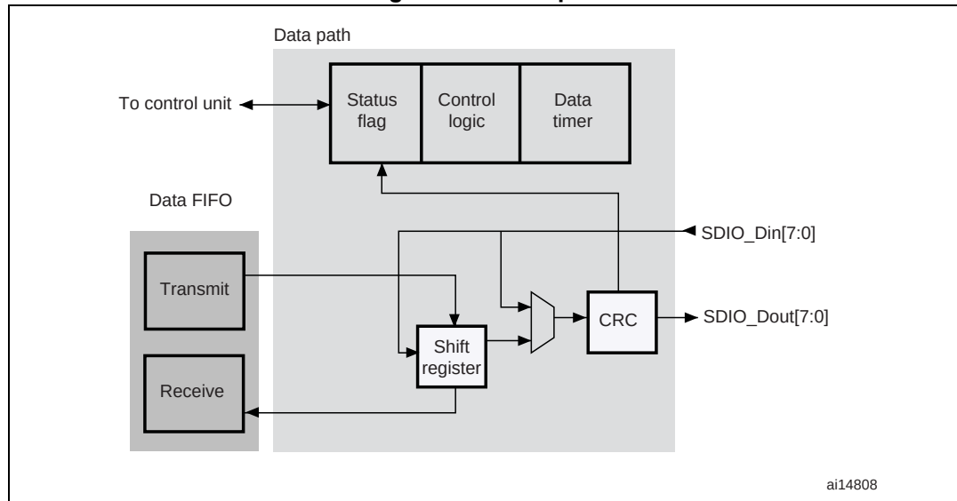
Figure 218. Data path
