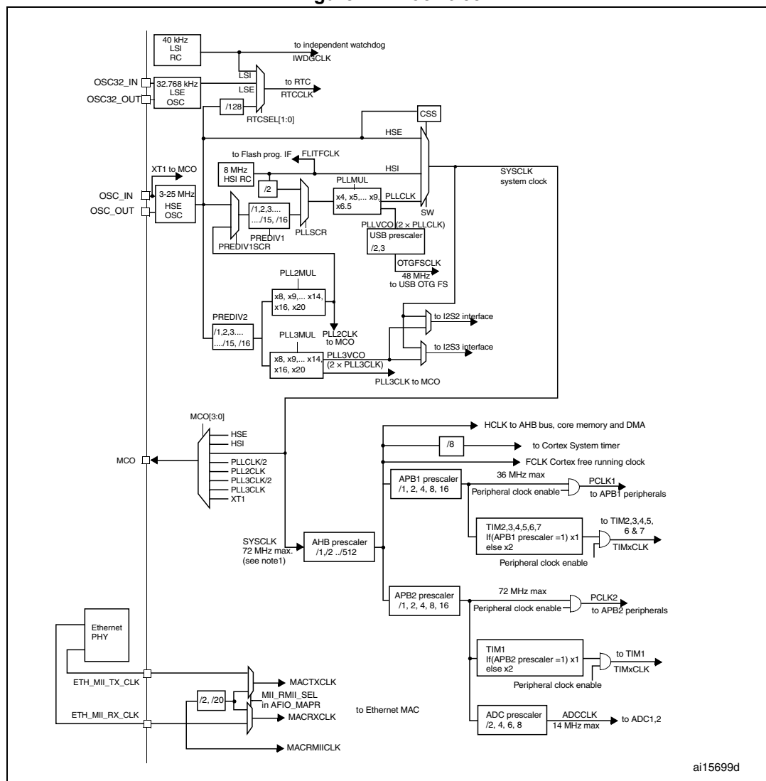
Figure 11. Clock tree
