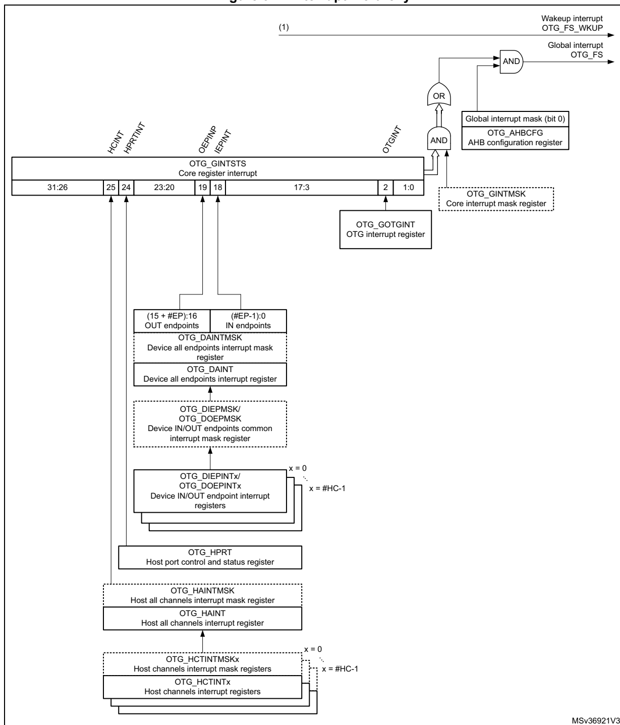
Figure 311. Interrupt hierarchy
