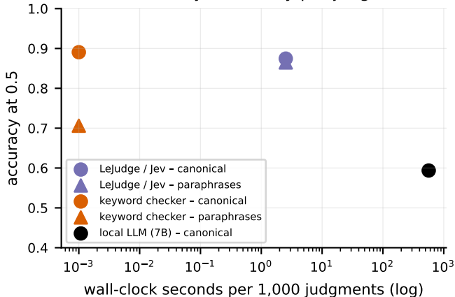
Accuracy vs latency per judge
