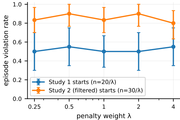
\lambda sweep, Jev, spatial set (95% bootstrap CIs)
