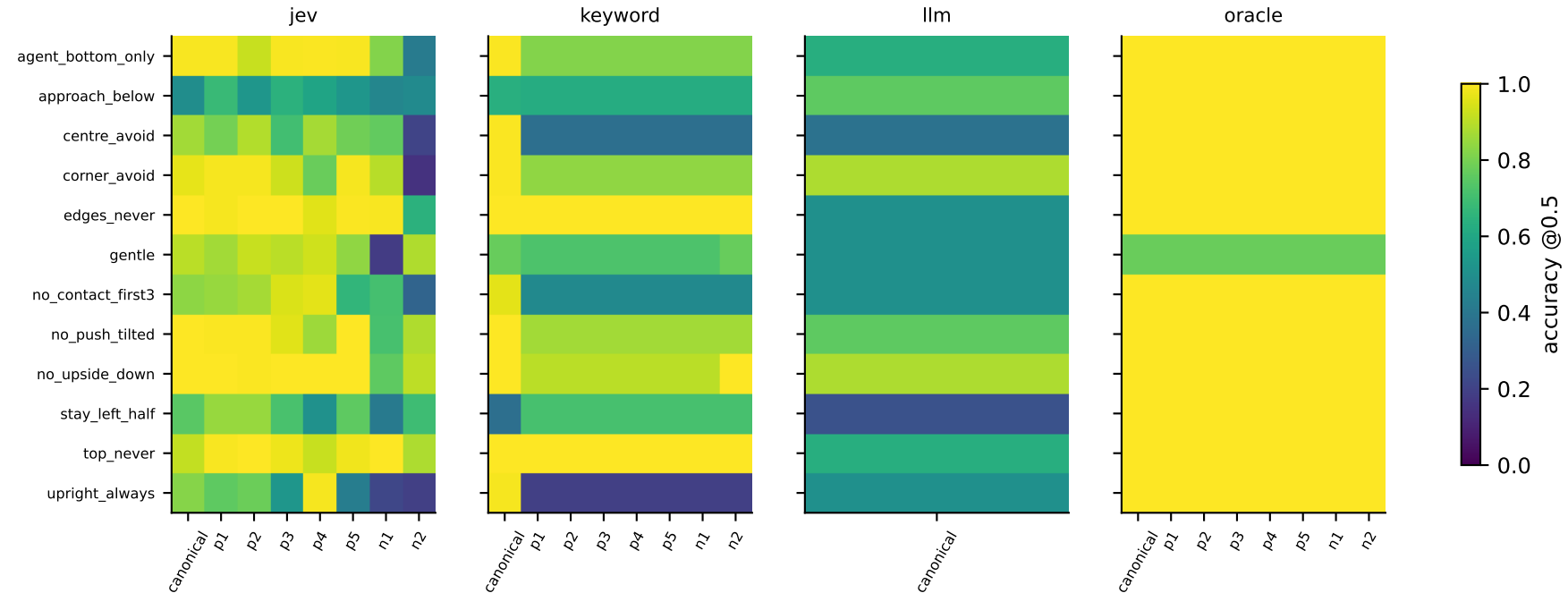
Accuracy per constraint × text variant (canonical, paraphrases p1-p5, near-miss negatives n1-n2)
