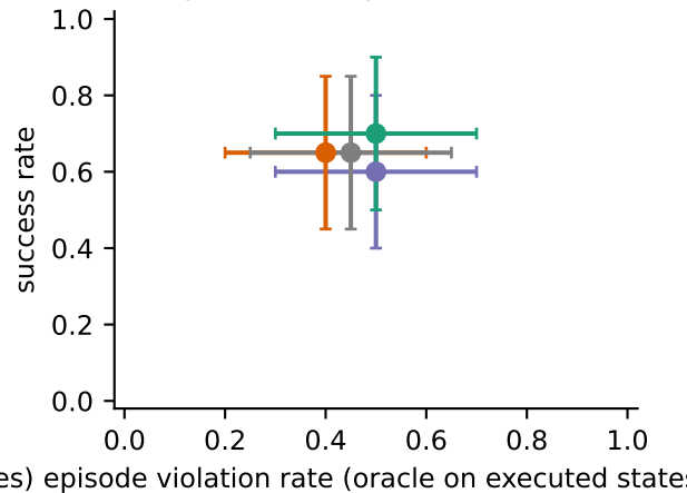
set: spatial+temporal (n=20/cond)
