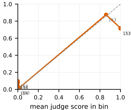
keyword checker, imagined items ECE = 0.089
