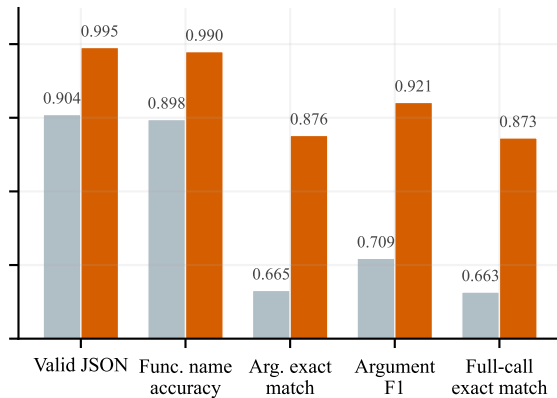
(b) French, n=879
