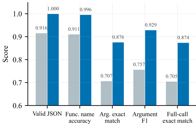
(a) English, n=1,000
