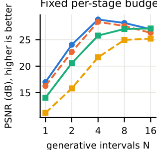
Fixed per-stage budget M = 40
