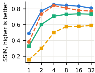
Fixed total budget B = N \times M = 160
