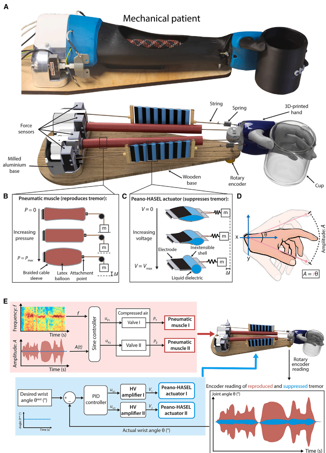
Figure 2. Design and control of the mechanical patient and tremor-suppression mechanism
