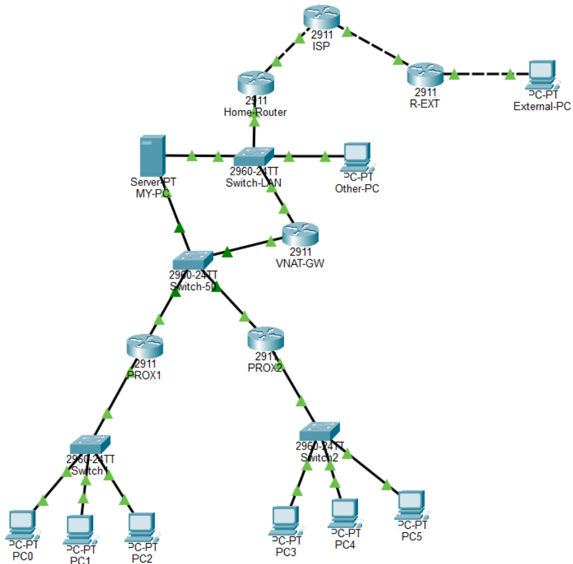
Figure 36: Simulated Network Topology - Cisco Packet Tracer
