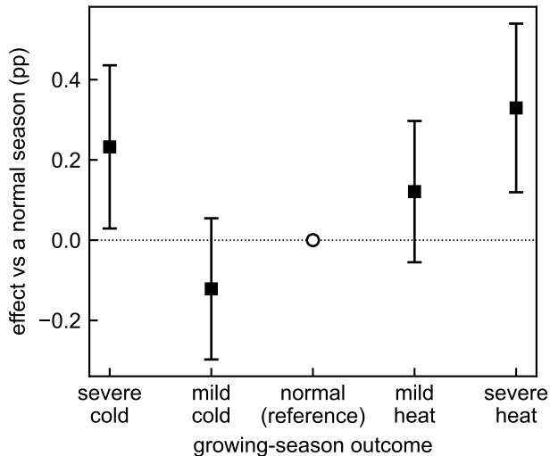
(a) Nonparametric bin response, h = 6
