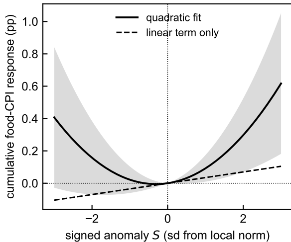
(b) Fitted shape, h = 6
