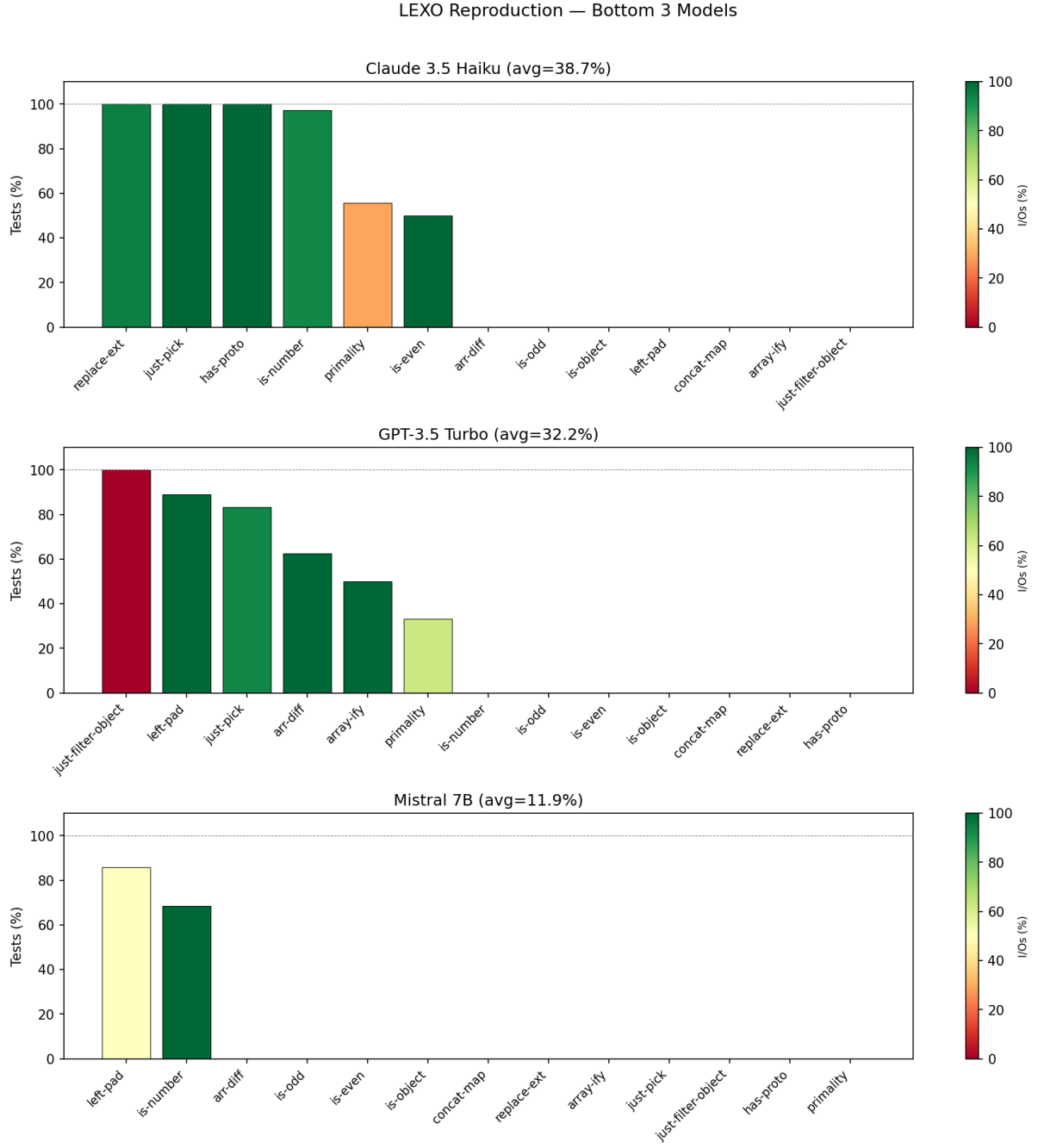
Figure 2: Bottom 3 models. Same axes.
