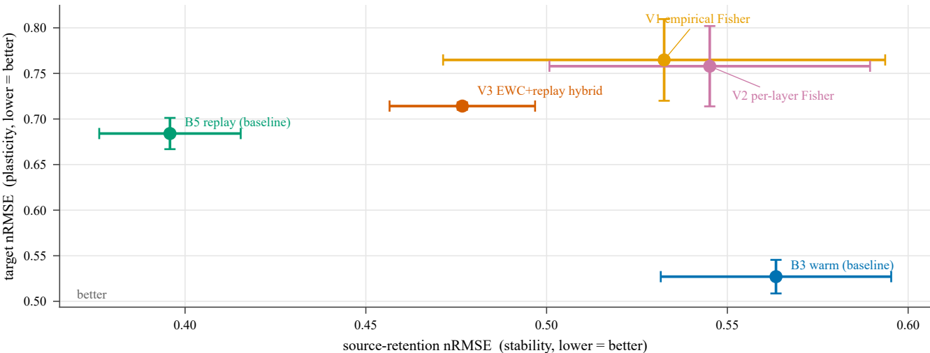
EWC-variants bench — none beats warm-start or replay (N=30, 3 seeds)
