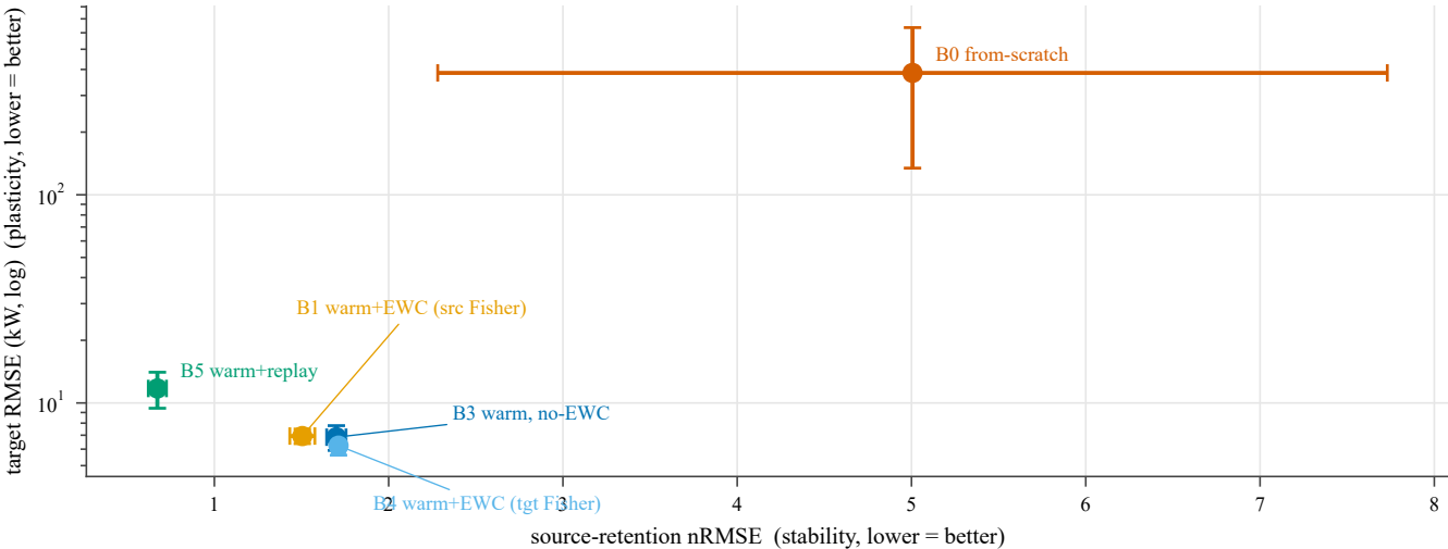
PV RQ2 --- stability--plasticity trade-off (N=30, 3 seeds)
