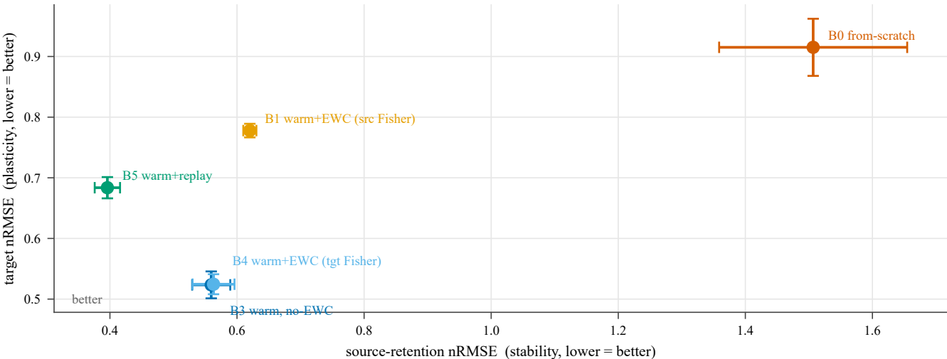
RQ2 — stability–plasticity tradeoff (N=30, 3 seeds)
