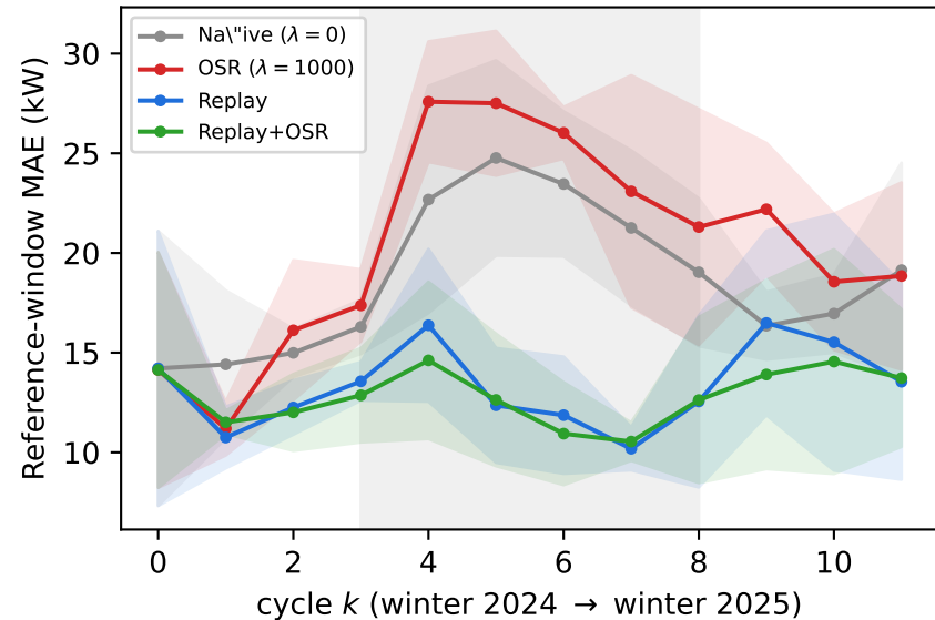
(a) Retention on fixed winter-2024 window
