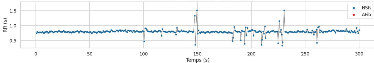
Transition NSR ↔ AFib (AFDB) — record 05121
