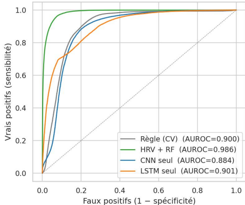
Courbes ROC — OOF AFDB 5-fold patient
