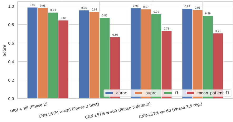
Phase 3.5 vs floor HRV+RF et Phase 3 (5-fold patient OOF, AFDB)
