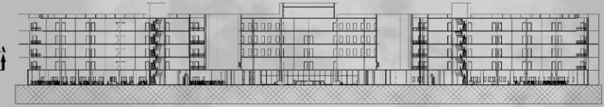
Section B-B Scale 1:200
