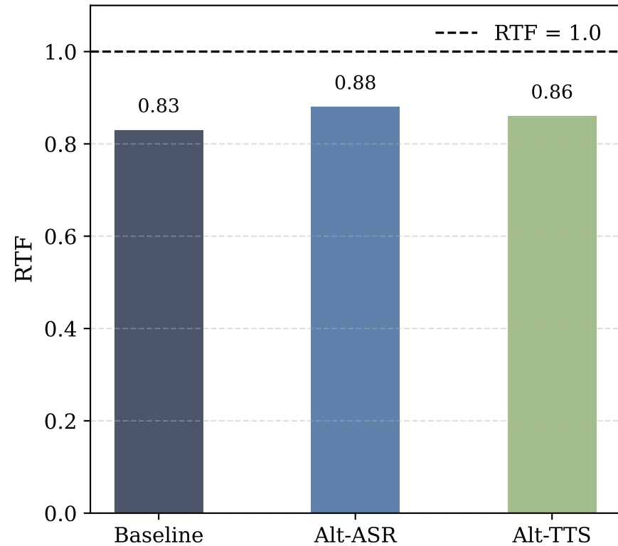
(c) Real-Time Factor (RTF)
