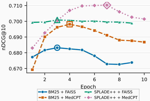
Dev nDCG@10
