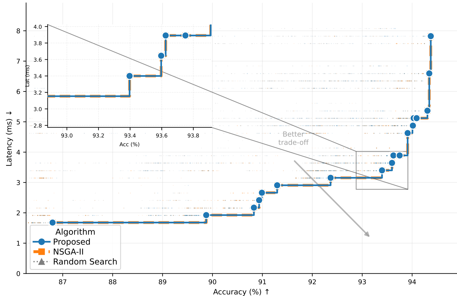
Pareto Front — cifar10 / Eyeriss Latency
