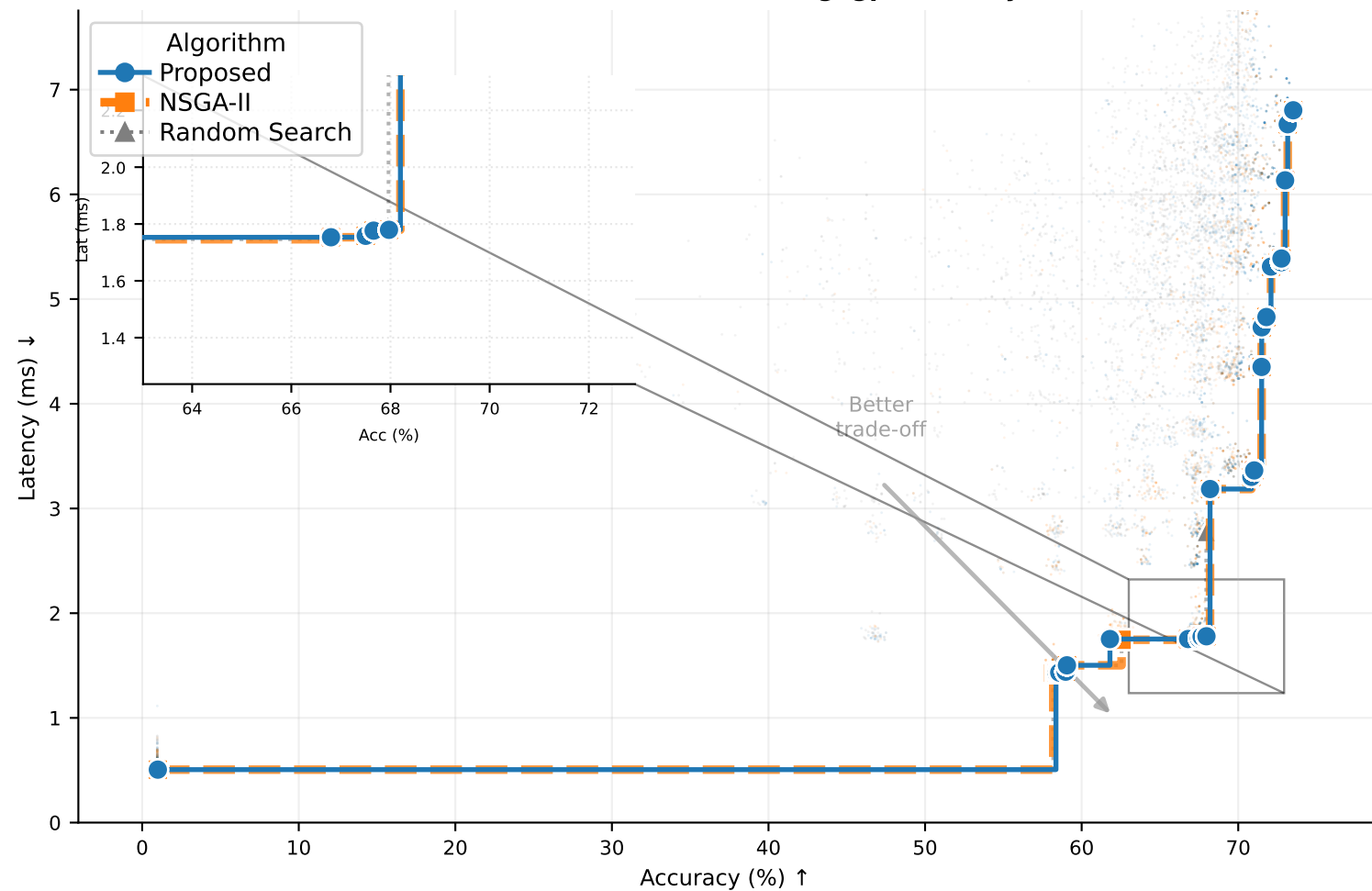
Pareto Front — cifar100 / Edgegpu Latency
